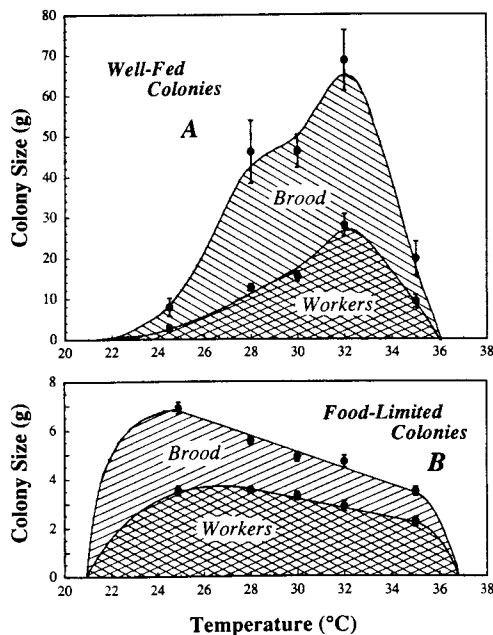
Fig. 2A, B. Effects of temperature on the size of A well-fed colonies and B food-limited colonies after 2 months (note difference in scales for colony size). Each figure shows total colony weight separated into worker and brood portions. Lines were fitted by eye and means are shown \pm 1 SE
