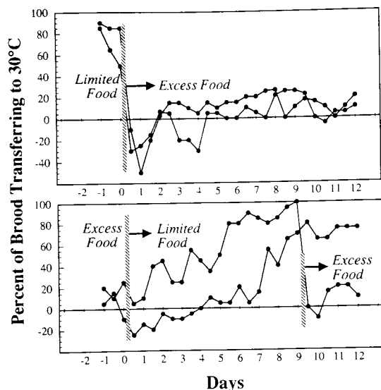
Fig. 5. Temporal change in thermal preferences of two fire ant colonies ( Solenopsis invicta ) switched from limited to excess food (top) and two colonies switched from excess to limited food (bottom). One colony in the bottom figure was switched back to excess food on day 9. Each line plots the percent of brood transferred from 32° C to 30° C with each 12-h switch in chamber temperature (a negative value indicates a net transfer to 32° C)
