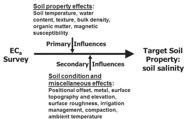
Fig. 5. Conceptual path diagram of the primary and secondary factors influencing an apparent soil electrical conductivity ( EC_a ) survey targeted at measuring soil salinity (source: modified from Corwin and Lesch, 2013).
