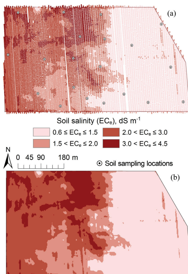
Fig. 12. Soil salinity (a) estimated using Eq. [11] at the 16122 soil apparent electrical conductivity survey locations and (b) interpolated on a 2 \times 2\ m block support for a 32.4-ha field near San Jacinto, CA.
