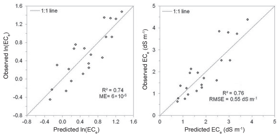
Fig. 11. Observed versus predicted (a) natural logarithm transformed soil salinity ( EC_e ) calculated with Eq. [10] and (b) back-transformed EC_e for a 32.4-ha field near San Jacinto, CA. Soil salinity is represented by the electrical conductivity of a saturated soil paste extract ( EC_e , dS m^{-1} ). R^2 is the coefficient of determination, ME is the mean error, and RMSE is the root mean square error. Dashed line is a 1:1 relationship.
