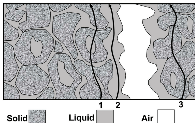
Fig. 2. Schematic illustrating the three conductance pathways for the apparent soil electrical conductivity ( EC_a ) measurement (modified from Rhoades et al., 1989). Pathway 1 is the solid-liquid conductance pathway, Pathway 2 is the liquid conductance pathway, and Pathway 3 is the solid conductance pathway.
