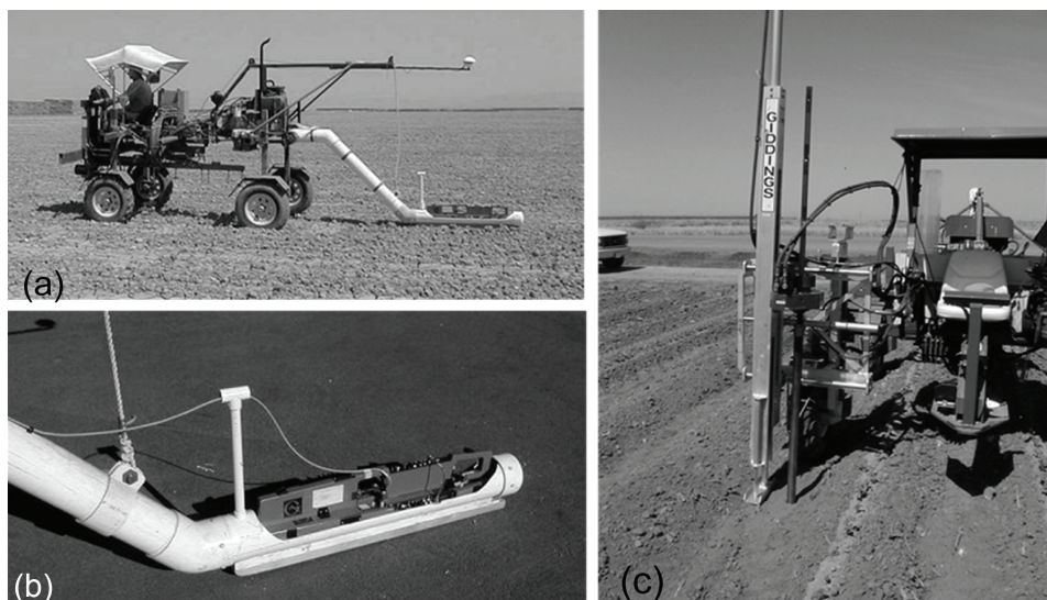
Fig. 3. Mobile electromagnetic induction equipment (source: Corwin and Lesch, 2005b): (a) complete rig; (b) close-up of sled holding the Geonics dual-dipole EM-38 soil electrical conductivity meter; and (c) close-up of Giddings soil core sampler.
