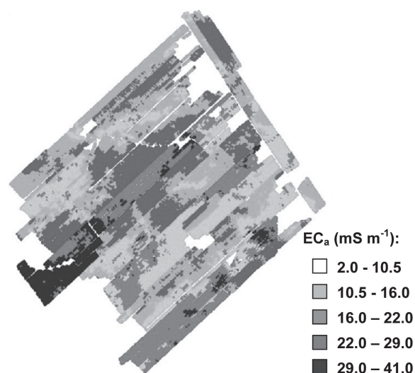
Fig. 9. Illustration of the “banding effect,” which is characteristic of a failed apparent soil electrical conductivity ( EC_a ) survey of soil salinity, resulting from the disregard of primary (e.g., water content, bulk density, temperature, texture) and secondary influences (e.g., surface roughness, presence of beds and furrows, compaction due to heavy equipment) effecting EC_a (source: Corwin and Lesch, 2013).
