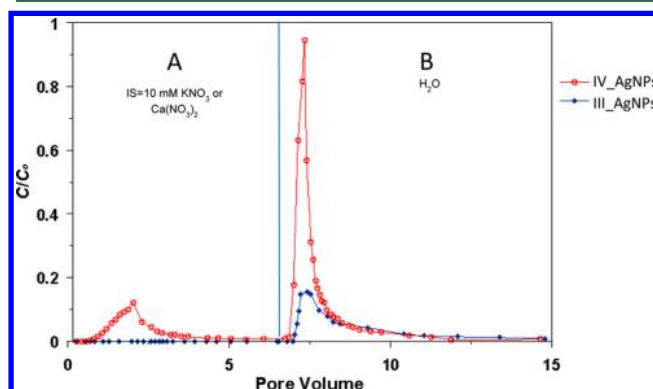
Figure 4. Breakthrough and release behavior of AgNPs in an undisturbed loamy sand soil. Deposition (step A) occurred at an IS = 10 mM using \text{Ca}(\text{NO}_3)_2 (experiment III) or \text{KNO}_3 (experiment IV), whereas release (step B) was initiated by eluting with Milli-Q water. The Darcy velocity was 0.02 cm/min and the input AgNP concentration was 10 mg/L.
