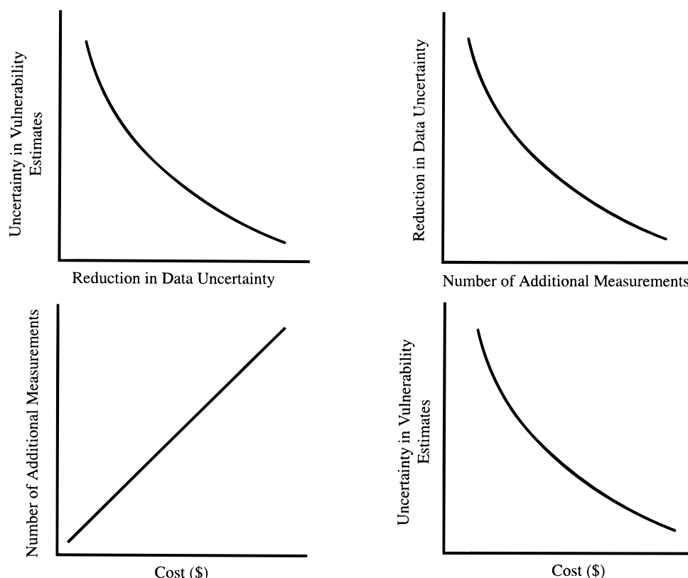
FIGURE 5. Schematic illustration of the general relationship between the cost of variance reduction and the efficiency of GIS-based NPS pollution models.
