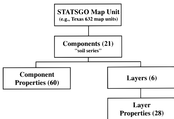
FIGURE 1. Structural hierarchy of the STATSGO soil database (154).
