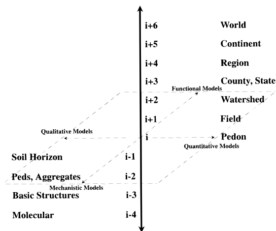
FIGURE 4. Organizational hierarchy of spatial scales pertinent to NPS pollutant models (238).
