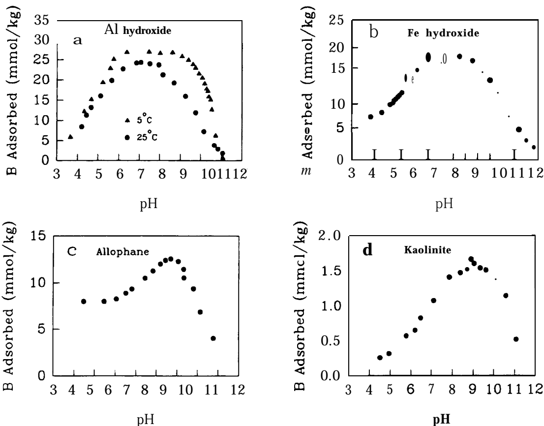
FIGURE 1. Boron adsorption in 0.1 M NaCl as a function of pH on (a) \text{am-Al(OH)}_3 , (b) \text{am-Fe(OH)}_3 , (c) allophane, and (d) kaolinite. The initial B concentration was approximately 0.462 \text{ mmol L}^{-1} .
