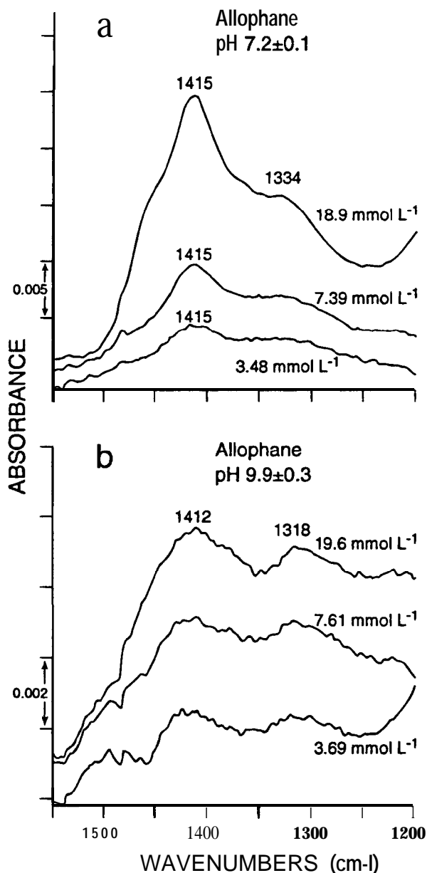
FIGURE 7. ATR-FTIR difference spectra of allophane paste at 25 \text{ }^\circ\text{C} : (a) in 0.1 \text{ M NaCl} with R = 8.18 \pm 0.06 ( n = 4 ) at pH 7.2 \pm 0.1 . The equilibrium B concentrations of 3.48 , 7.39 , and 18.9 \text{ mmol L}^{-1} correspond to \Gamma = 65 \text{ mmol kg}^{-1} and \theta = 28\% ; \Gamma = 109 \text{ mmol kg}^{-1} and \theta = 23\% ; and \Gamma = 247 \text{ mmol kg}^{-1} and \theta = 21\% , respectively; (b) in 0.1 \text{ M NaCl} with R = 8.30 \pm 0.06 at pH 9.9 \pm 0.3 . Values of C_e of 3.69 , 7.61 , and 19.6 \text{ mmol L}^{-1} correspond to \Gamma = 49 \text{ mmol kg}^{-1} and \theta = 35\% ; \Gamma = 85 \text{ mmol kg}^{-1} and \theta = 30\% ; and \Gamma = 181 \text{ mmol kg}^{-1} and \theta = 15\% , respectively.
