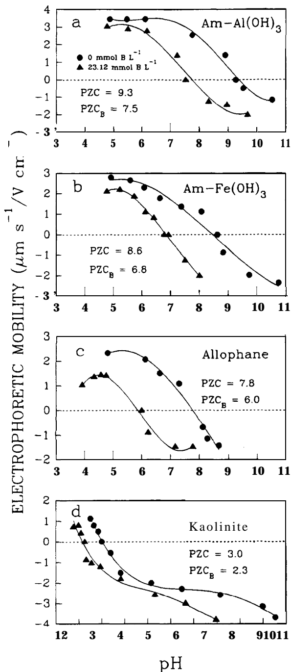
FIGURE 2. Effect of added boric acid on the electrophoretic mobility at 25 °C as a function of pH: (a) \text{am-Al(OH)}_3 , (b) \text{am-Fe(OH)}_3 , (c) allophane, and (d) kaolinite.
