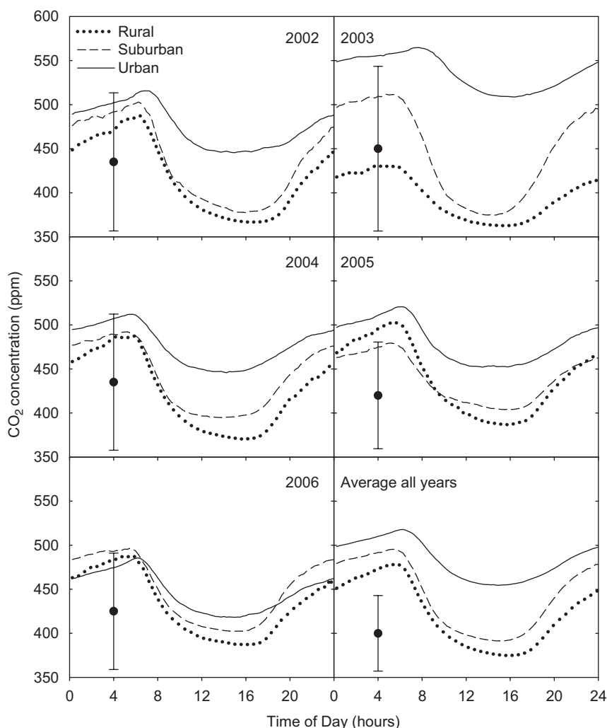
Fig. 2. Near surface atmospheric CO 2 concentration averaged over a 24 h period for each site along the transect for the 5 years of the study. Data were recorded every 15 min resulting in 96 values over a 24 h period consequently data points and error bars are not included but the data are connected by straight lines. The error bars shown in each graph is the maximum standard deviation from all sites.
