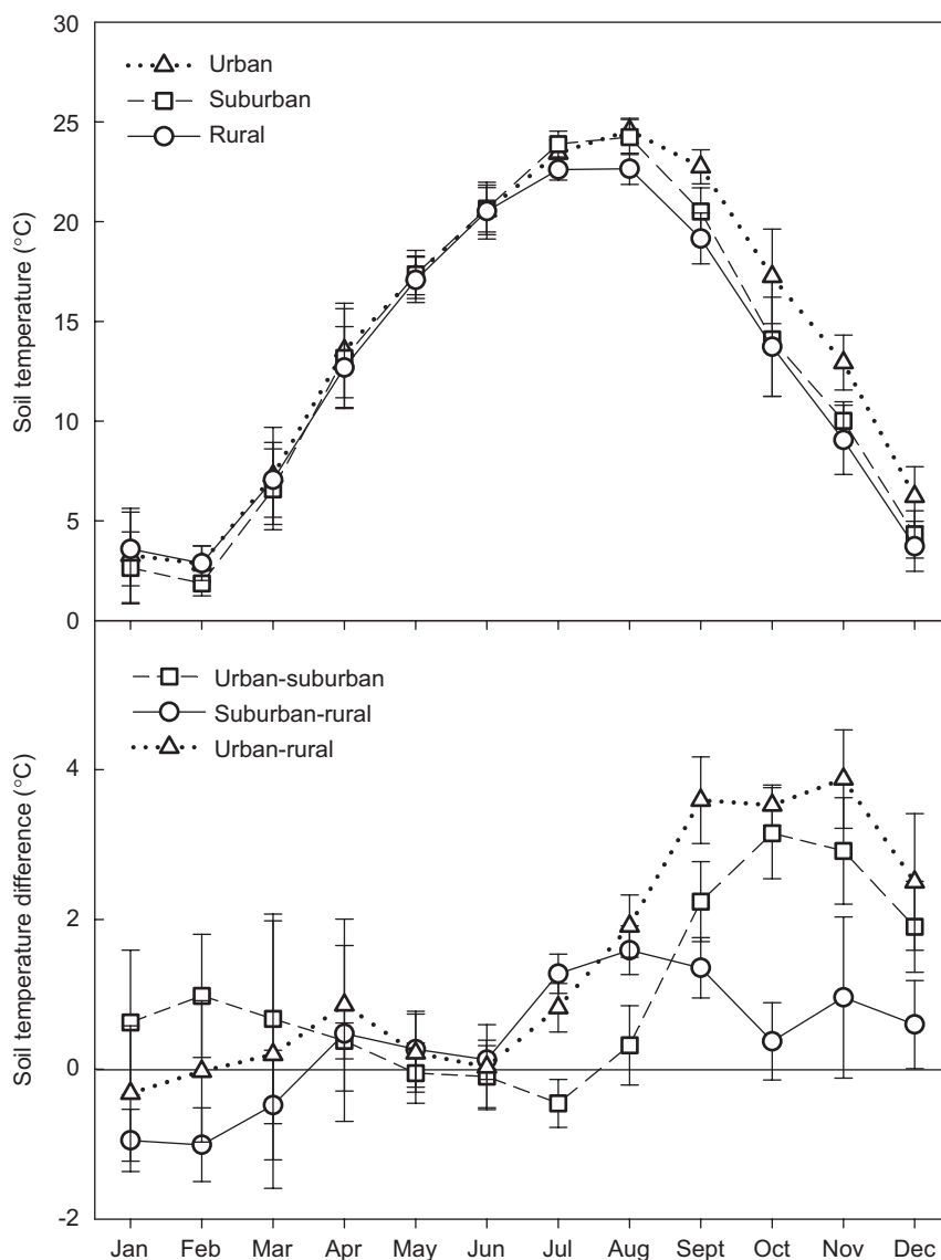
Fig. 4. Annual soil temperature (10 cm depth) averaged over the 5 years of the study and differences between sites on a monthly basis. The error bars are one standard deviation.
