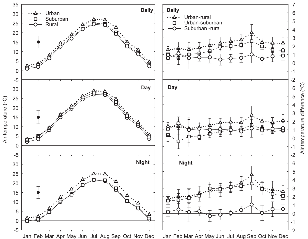
Fig. 3. Daily (24h), daytime and nighttime air temperature for each site along the transect averaged over the 5 years of the study. The error bars for the graphs on the left side are the maximum standard deviation. The graphs on the right represent the deviations in temperature between sites, the error bars are one standard deviation.
