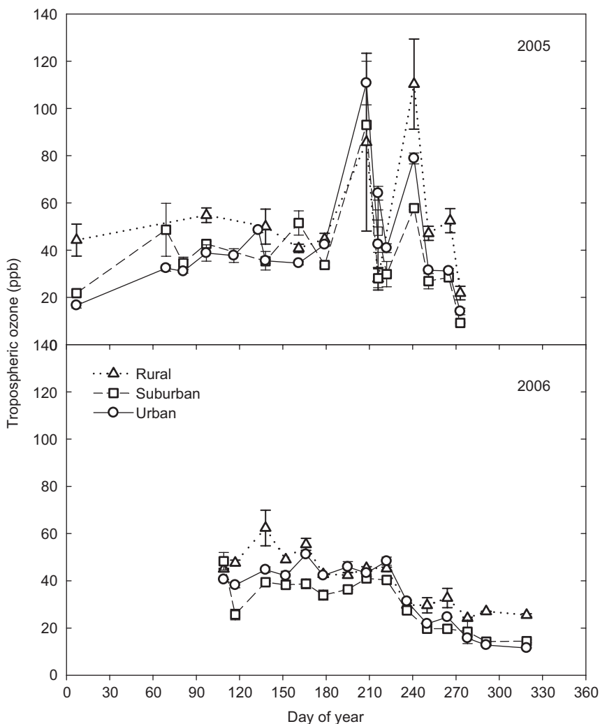
Fig. 5. Tropospheric ozone measured at each site through the growing season of 2005 and 2006. The error bars are one standard deviation.
