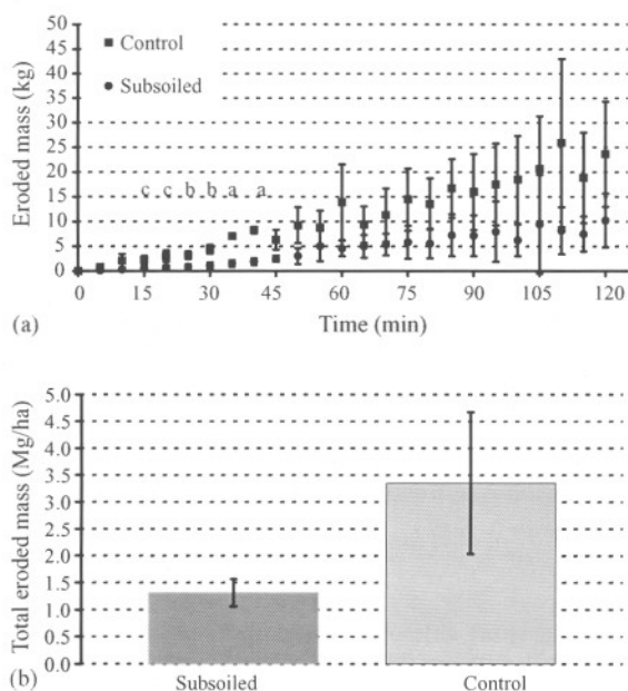
Fig. 4. Eroded material averages and standard errors ( n = 4 ) from simulated rainfall plots. (A) Mass of eroded soil (kg) mass from plots at 5 min intervals following initiation of flow. Letters above incremental data points indicate significance of difference between treatments: a, \alpha \leq 0.01 ; b, \alpha \leq 0.05 ; c, \alpha \leq 0.10 . (B) Total eroded material (Mg/ha) from 51 \pm 1 mm of simulated rainfall.
