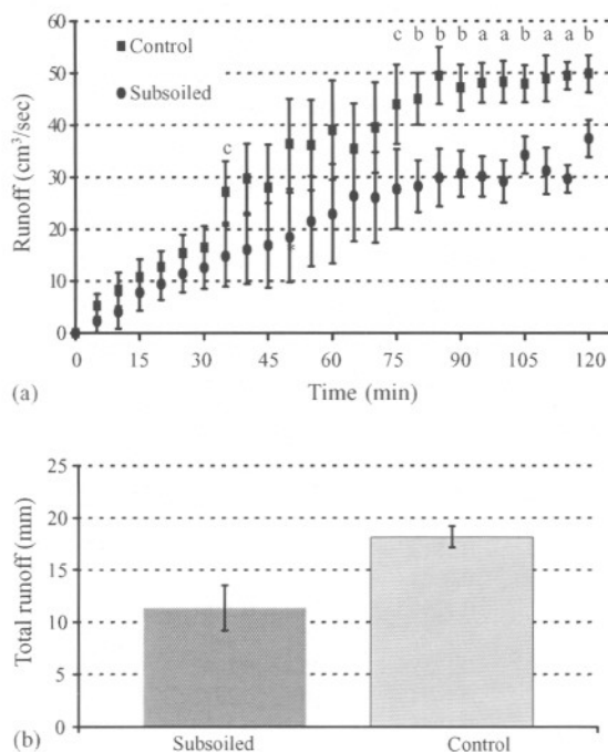
Fig. 3. Runoff averages and standard errors ( n = 4 ) from the first 2 h of simulated rainfall on rotary-subsoiled and control treatments at Harrington. (A) Runoff rates in cubic centimeters per second from plots at 5 min intervals following initiation of flow. Letters above incremental data points indicate significance of difference between treatments: a, \alpha \leq 0.01 ; b, \alpha \leq 0.05 ; c, \alpha \leq 0.10 . (B) Total runoff from 51 ± 1 mm of simulated rainfall.
