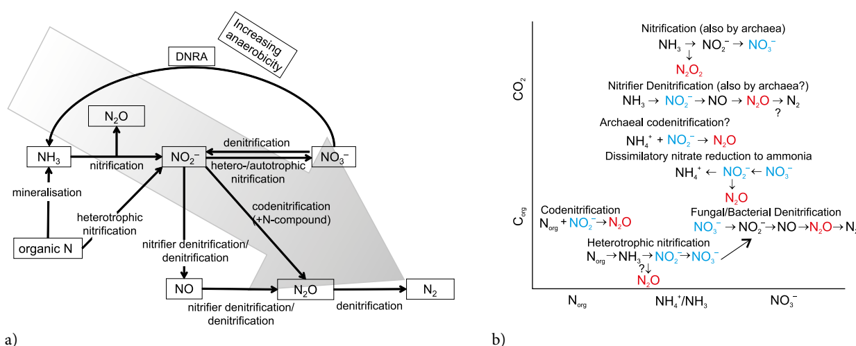
Fig. 1. a) Processes and b) pathways of N conversions associated with \text{N}_2\text{O} emissions in soils in relation to N transformations (A) and N and C substrates (B). (Figure credit: N. Wrage-Mönnig)
