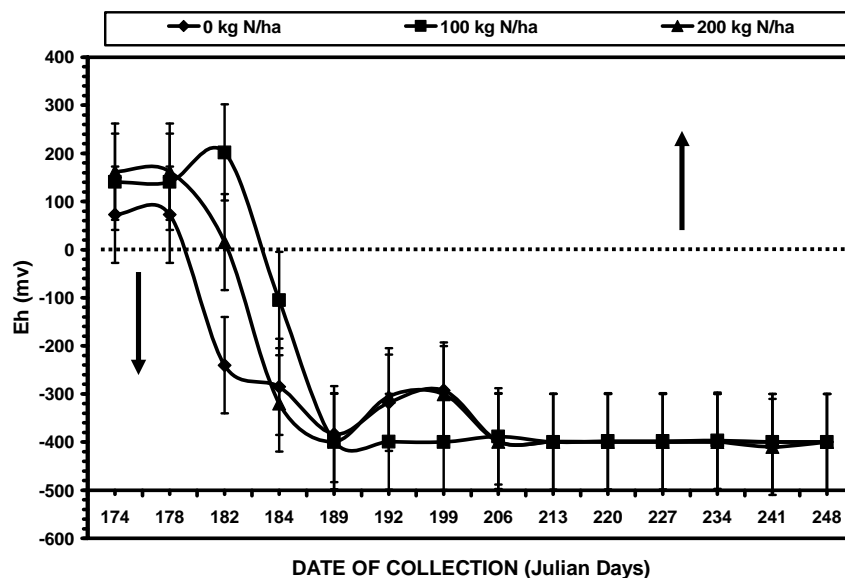
Figure 1. Average levels of reduction-oxidation (Eh) readings during the flooding experiment.
