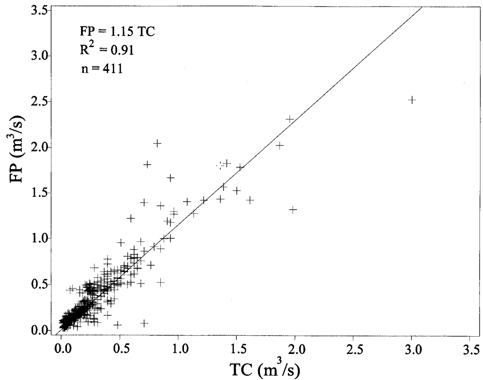
Figure 2-Regression of Flow-Proportional (FP) and Time Composed (TC) flow measurements.
