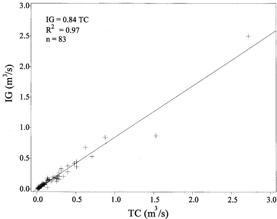
Figure 3—Regression of Instantaneous Grab Sample (IG) and Time Compositd (TC) flow measurements.
