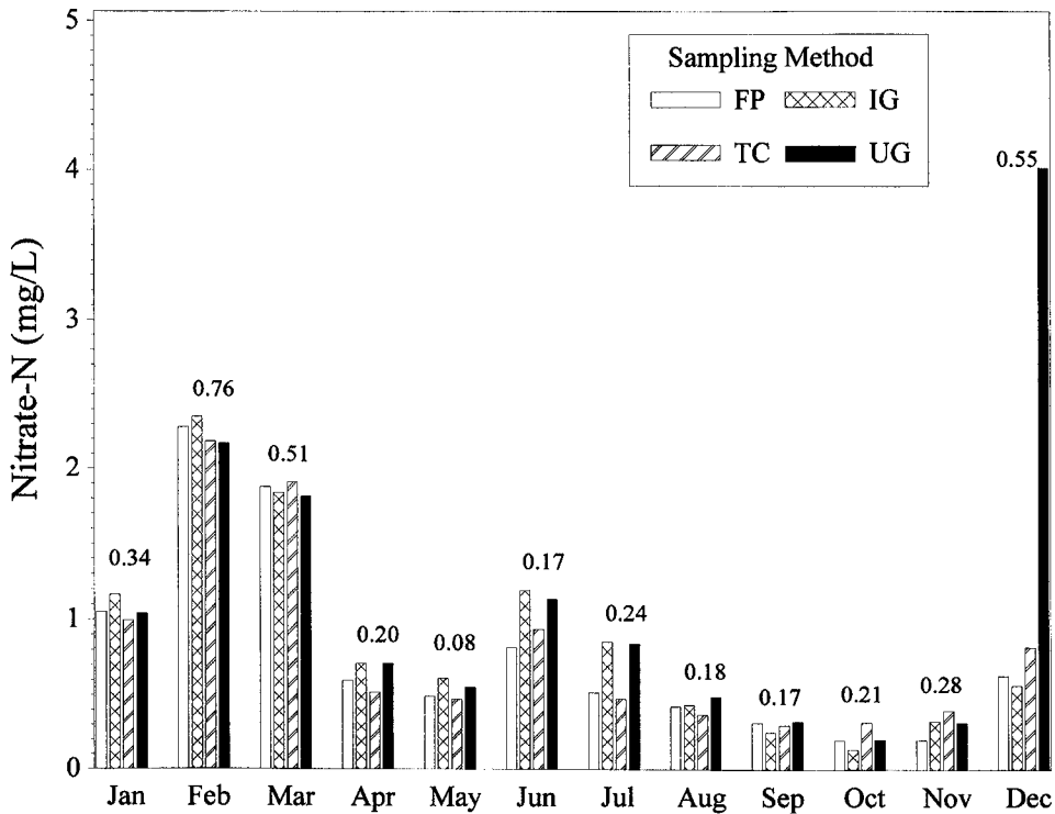
Figure 5—Mean 1995 monthly nitrate-N concentrations for the Herrings Marsh Run watershed for the four sampling methods (LSD 0.05 values are shown above each month).
