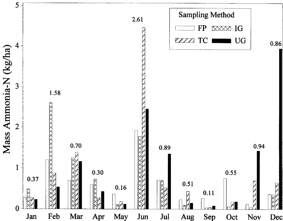
Figure 8—Mean 1995 monthly mass ammonia-N loadings for the Herrings Marsh Run watershed for the four sampling methods (LSD 0.05 values are shown above each month).
