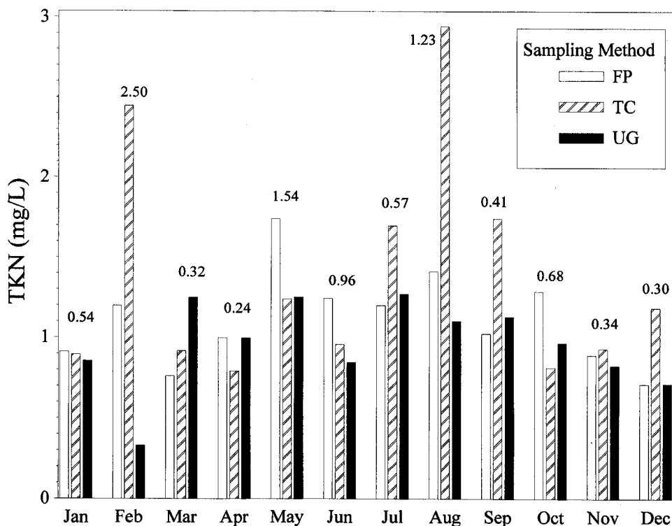
Figure 9—Mean 1995 monthly TKN concentrations for the Herrings Marsh Run watershed for three sampling methods (LSD 0.05 values are shown above each month).
