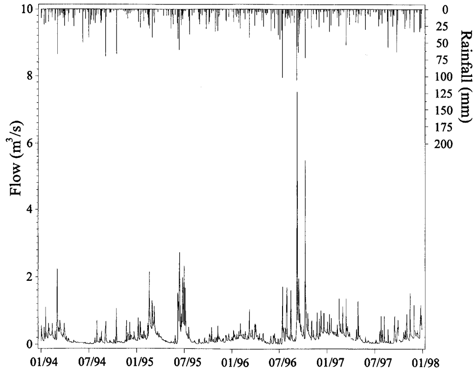
Figure 1-USGS stream flow and rainfall for the Herring Marsh Run watershed.
