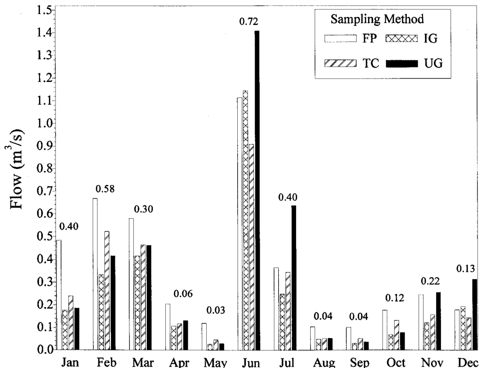
Figure 4—Mean 1995 monthly flow measurements for the Herring Marsh Run watershed for the four sampling methods (LSD 0.05 values are shown above each month).
