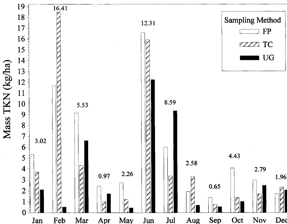
Figure 10—Mean 1995 monthly mass TKN loadings for the Herrings Marsh Run watershed for three sampling methods (LSD 0.05 values are shown above each month).
