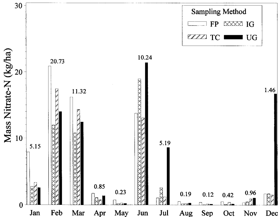
Figure 6—Mean 1995 monthly mass nitrate-N loadings for the Herrings Marsh Run watershed for the four sampling methods (LSD 0.05 values are shown above each month).
