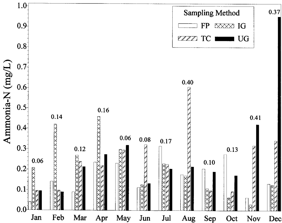
Figure 7—Mean 1995 monthly ammonia-N concentrations for the Herrings Marsh Run watershed for the four sampling methods (LSD 0.05 values are shown above each month).
