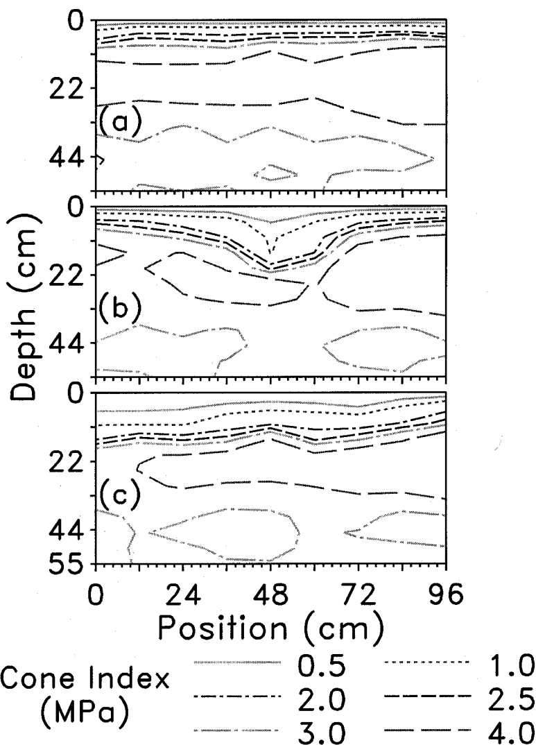
Figure 1. Soil cone index contours for plots with laterals and tillage treatments of (a) no tillage, (b) tillage with the Beasley, and (c) tillage with the Stubble Mulcher.
