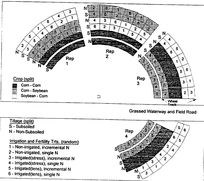
FIGURE 4. Plot plan for replicated field experiment used to test site-specific center pivot under controlled conditions. (After Sadler et al. , 1996).
