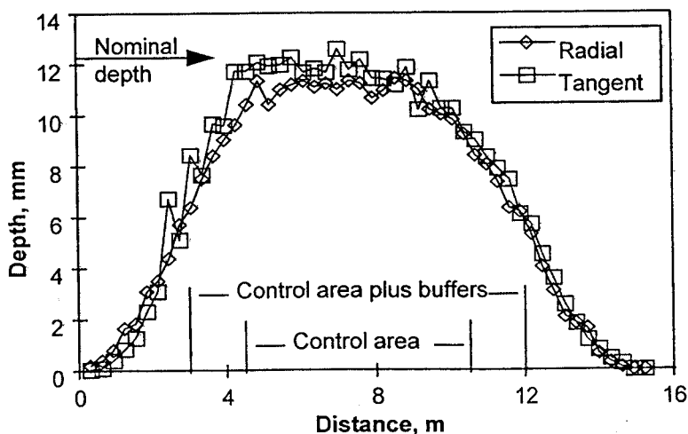
FIGURE 2. Radial and tangential distribution of application depth for a single element surrounded by unirrigated elements. Each point is the mean of three measurements.
