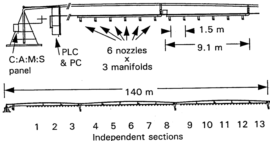
FIGURE 1. Side view of site-specific center pivot and closeup of tripod and example section.
