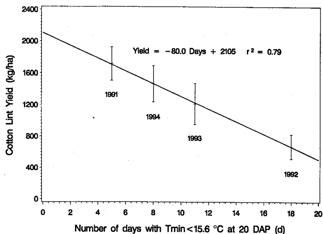
Figure 5—Relationship between cotton lint yield and number of days during the first 20 DAP with daily minimum temperature less than 15.6^{\circ}\text{C} each year for 1991-1994.
