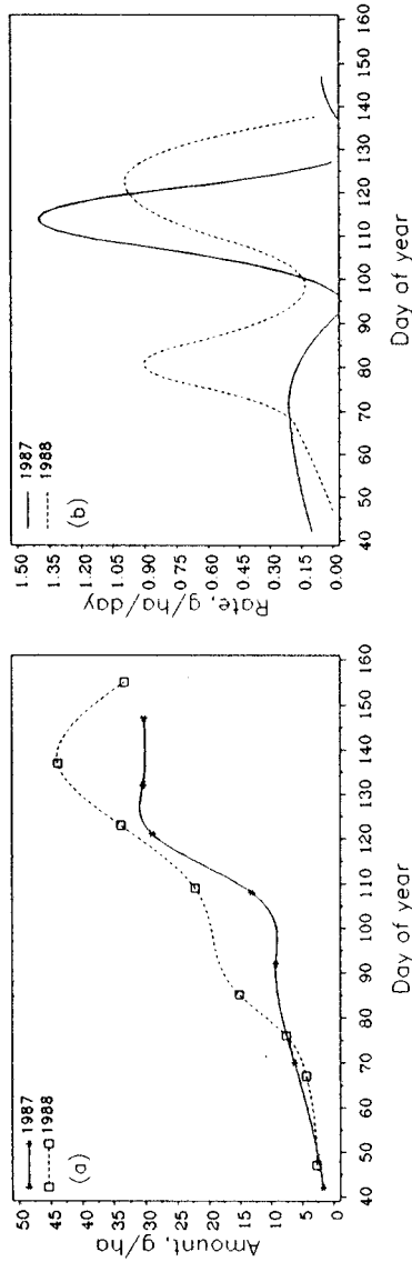
Figure 9. Amount (a) and rate (b) of aerial boron accumulation.
