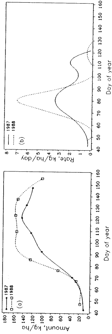
Figure 5. Amount (a) and rate (b) of aerial potassium accumulation.
