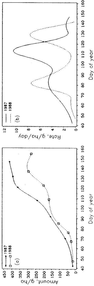
Figure 11. Amount (a) and rate (b) of aerial manganese accumulation.
