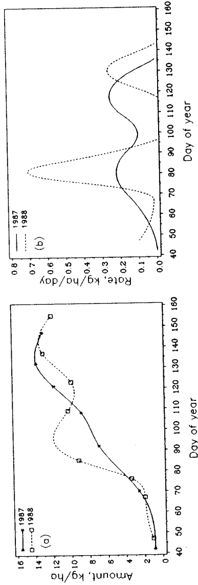
Figure 6. Amount (a) and rate (b) of aerial sulfur accumulation.
