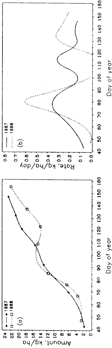
Figure 4. Amount (a) and rate (b) of aerial phosphorus accumulation.
