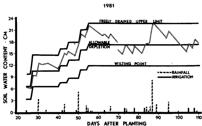
Fig. 6—Calculated soil-water content, irrigation, and rainfall for the CBWB treatment during the 1981 growing season. Wilting point is soil water retained at 1.5 MPa.
