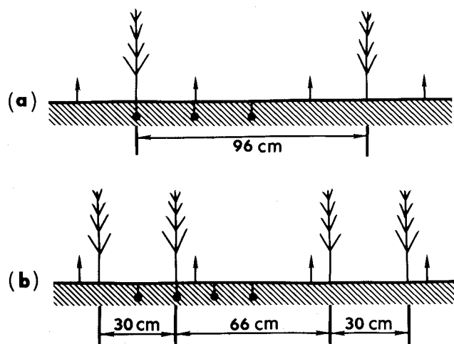
Fig. 1—Schematic diagram showing position of irrigation lines (vertical arrows), tensiometers (solid circles) and corn rows for (a) the single-row configuration and (b) the twin-row configuration.
