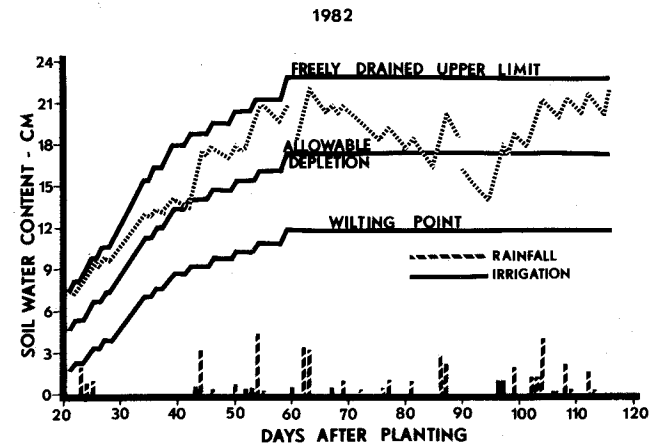
Fig. 7—Calculated soil-water content, irrigation, and rainfall for the CBWB treatment during the 1982 growing season. Wilting point is soil water retained at 1.5 MPa.
