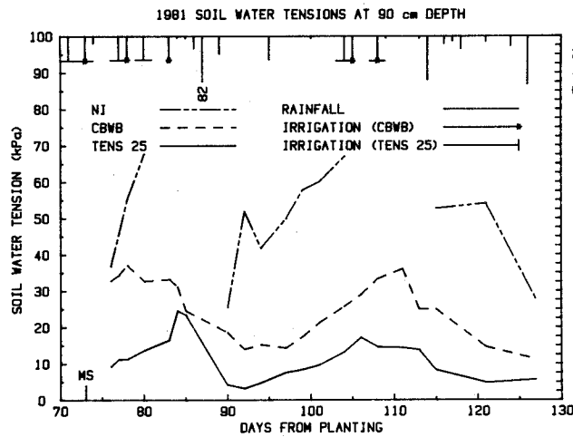
Fig. 4—Soil-water tension at the 30- (top) and 90-cm (bottom) depths for the NI and two irrigation treatments during the 1981 growing season. Numbers printed on daily rainfall lines reflect daily rainfall totals which exceeded the plotting range.
