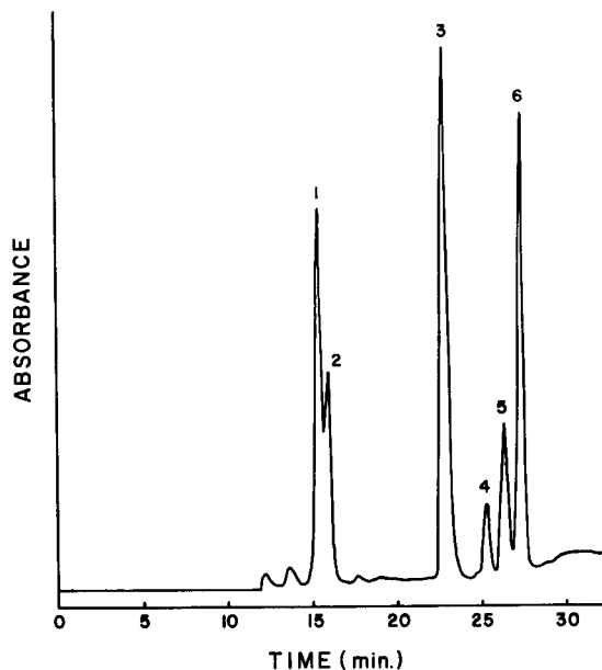
Figure 1. LC of phenolics from "Jewel" sweet potato (inner tissue). (1) Chlorogenic acid; (2) neochlorogenic acid; (3) coumarin (internal standard); (4) isochlorogenic acid A; (5) isochlorogenic acid B; (6) isochlorogenic acid C.
