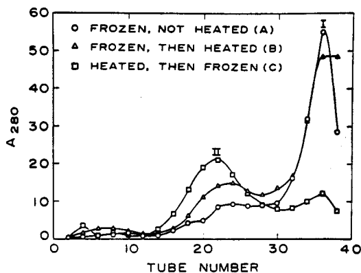
FIG. 2. Counter-current distribution profiles of ethyl acetate extracts of olives. Solvent system: top phase, ethyl acetate; bottom phase, 0.1 M potassium phosphate, pH 4.6. Band I contained inhibitory activity but no acid-hydrolyzable glycosides; compounds 5 and 6 from thin-layer chromatography were contained in this fraction. Band II contained a phenolic glucoside but no inhibitory activity; compounds 1 to 4 from thin-layer chromatography were contained in this fraction.
