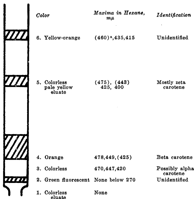
FIG. 2. Schematic chromatogram of carotene fraction from peanut oil on magnesium oxide columns after treatment with lithium aluminum hydride.
