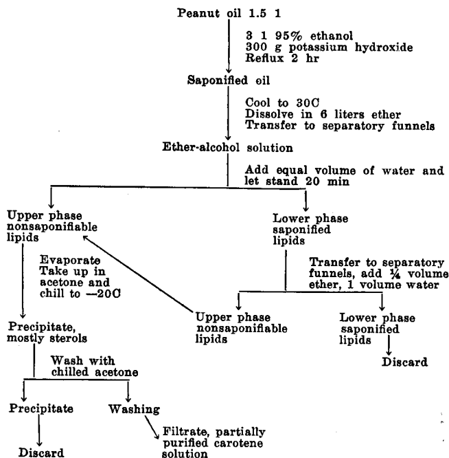
FIG. 1. Scheme for extracting carotenoids from peanut oil.
