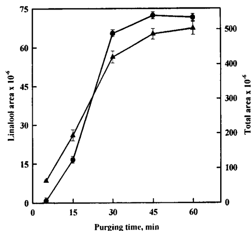
Figure 1. Effect of purging time on peak area of linalool (●) and total area (▲) of the total ion chromatogram excluding the area of the ethyl acetate, acetic acid, and internal standard peaks.
