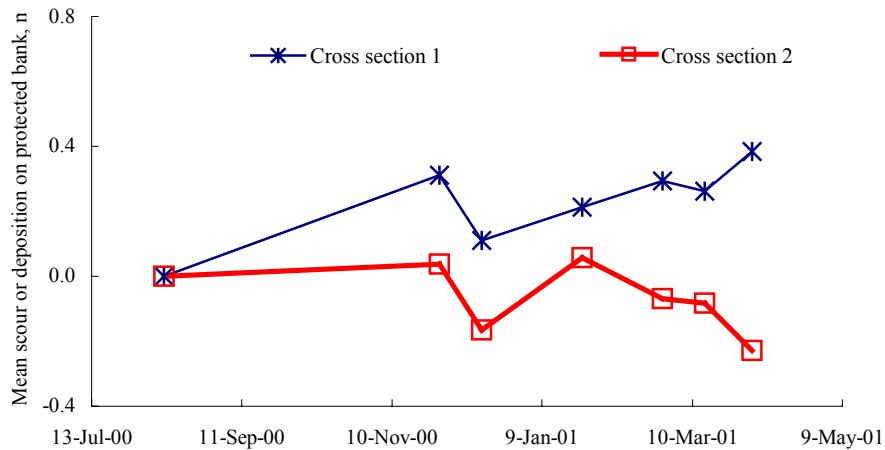
Figure 5. Average scour (-) or deposition (+) for bank protected by large woody debris along cross sections 1 and 2 shown in Figure 2. Scour and deposition were computed for segments of cross section between top bank and approximate streamward margin of large woody debris structure. Initial point (zero) represents conditions immediately following construction.
