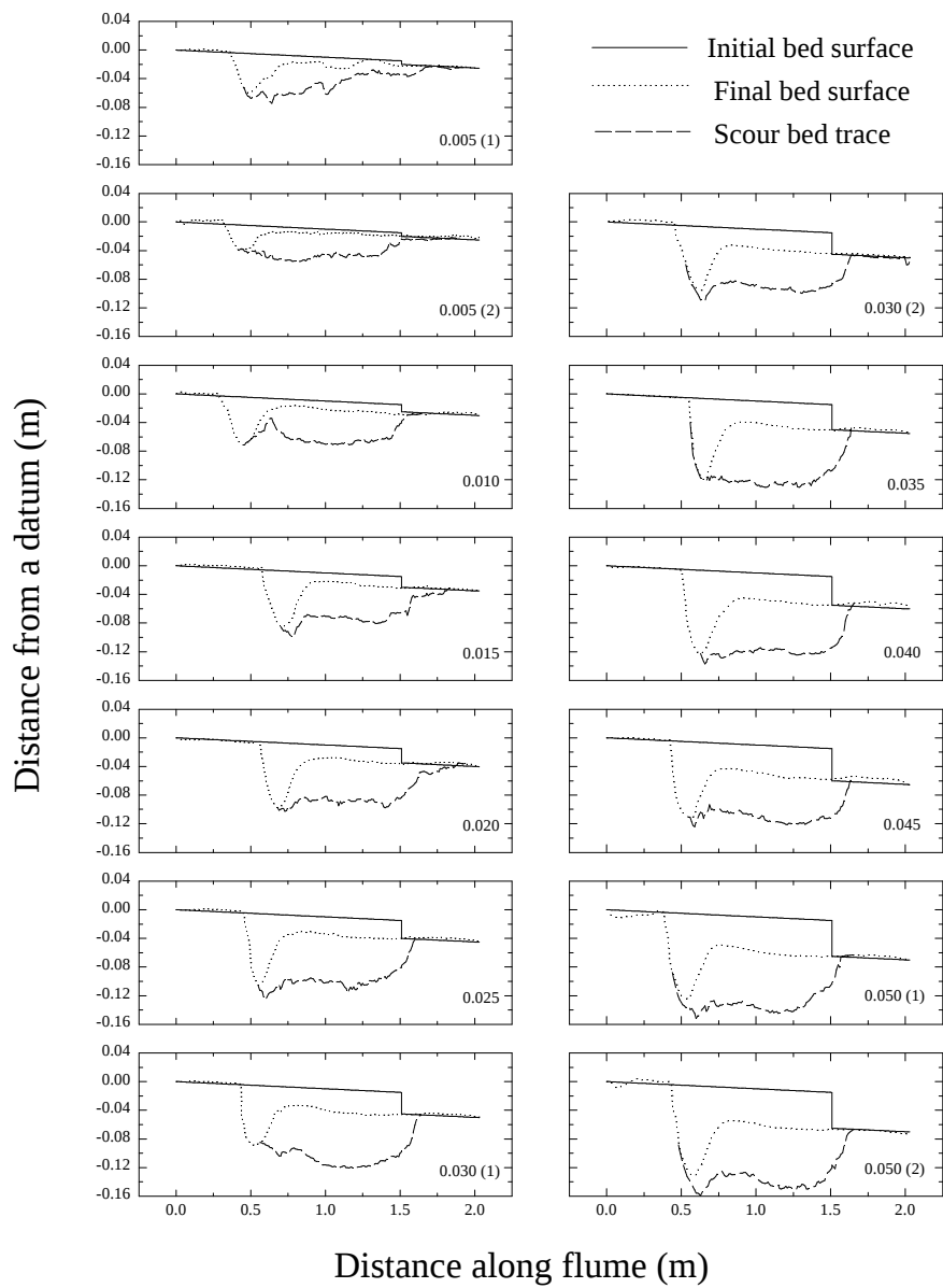
Along flume profiles of the initial and final bed surface, and the trace of the scour depth for all experiments. Flow is from left to right.
