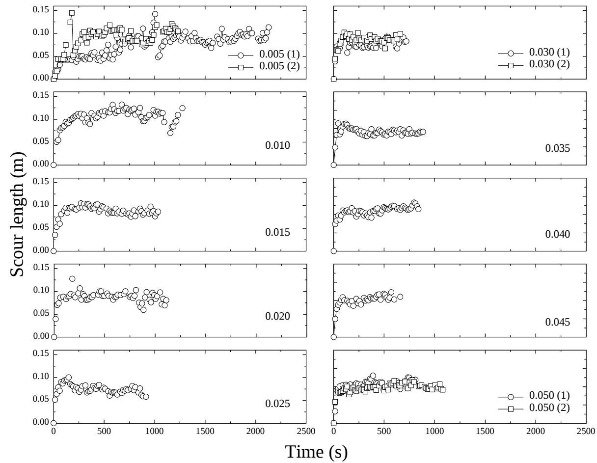
Time variation in headcut length at 15-s intervals.
