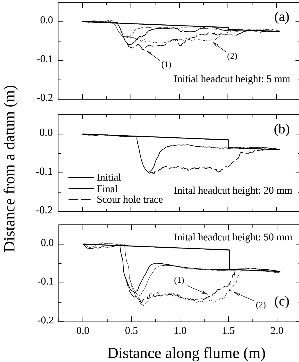
Figure 2. Along flume profiles of the initial and final bed surfaces and the trace of the scour depth for experiments with initial headcut heights of (a) 5, (b) 20, and (c) 50 mm. Flow is from left to right.
