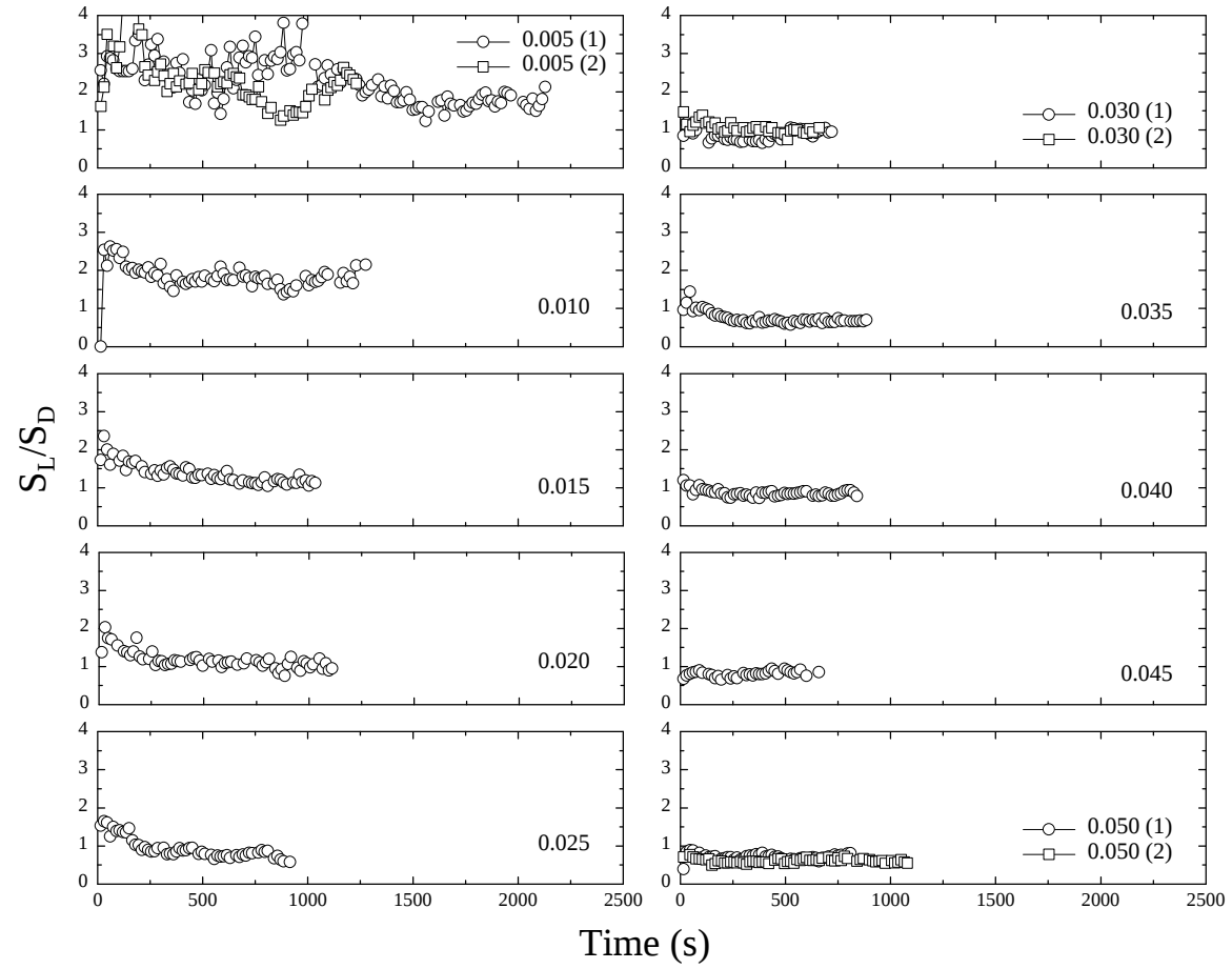
Time variation in the ratio of the length to the maximum scour depth-to-maximum scour depth S_L/S_D measured at 15-s intervals.
