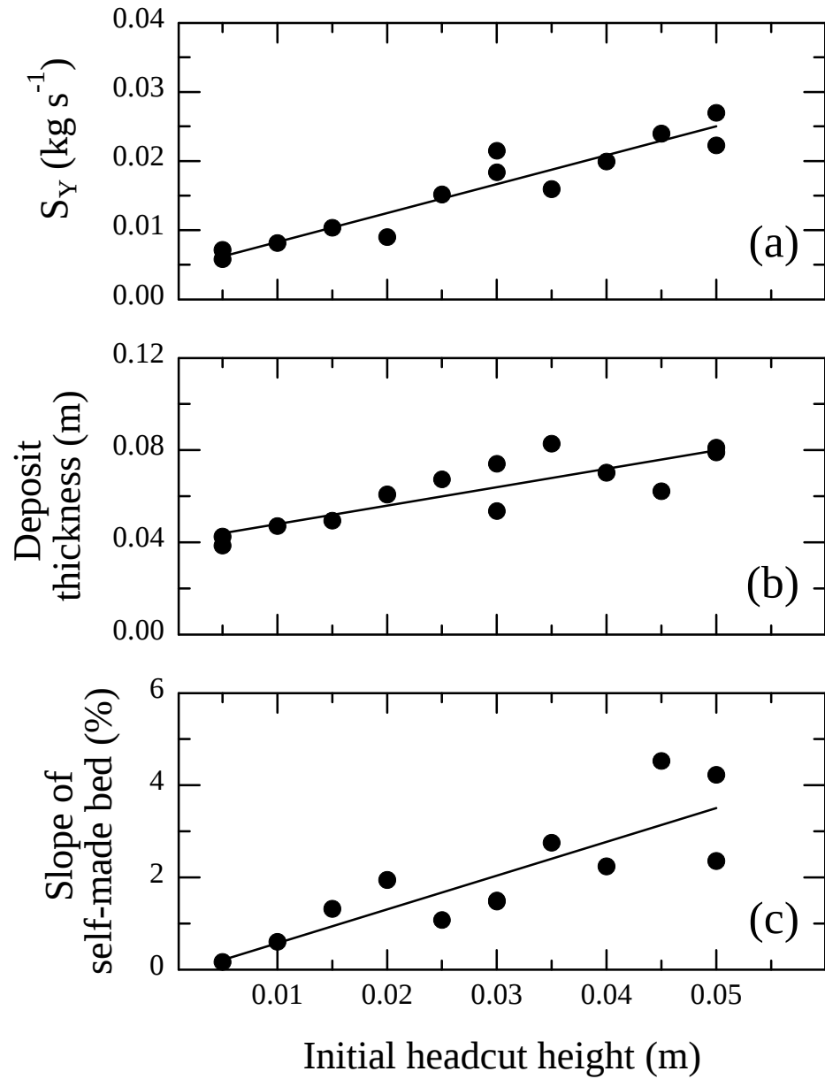
Figure 6. Variation of steady-state sediment transport parameters with initial headcut height. Shown are (a) sediment yield ( R=0.95 ; PW=1.0 ; using a=0.05 and P=0.001 ), (b) deposit thickness ( R=0.85 ; PW=0.98 , and (c) slope of self-made bed ( R=0.84 ; PW=0.96 ).
