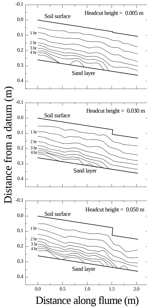
Procession of the wetting front through the soil profile as observed from the flume sidewall for runs 0.005(1), 0.030(2) and 0.050(1).
