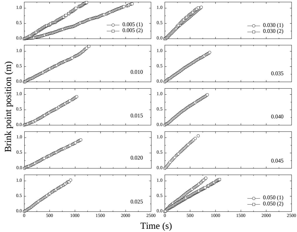
Time variation in headcut brinkpoint position measured at 15-s intervals.
