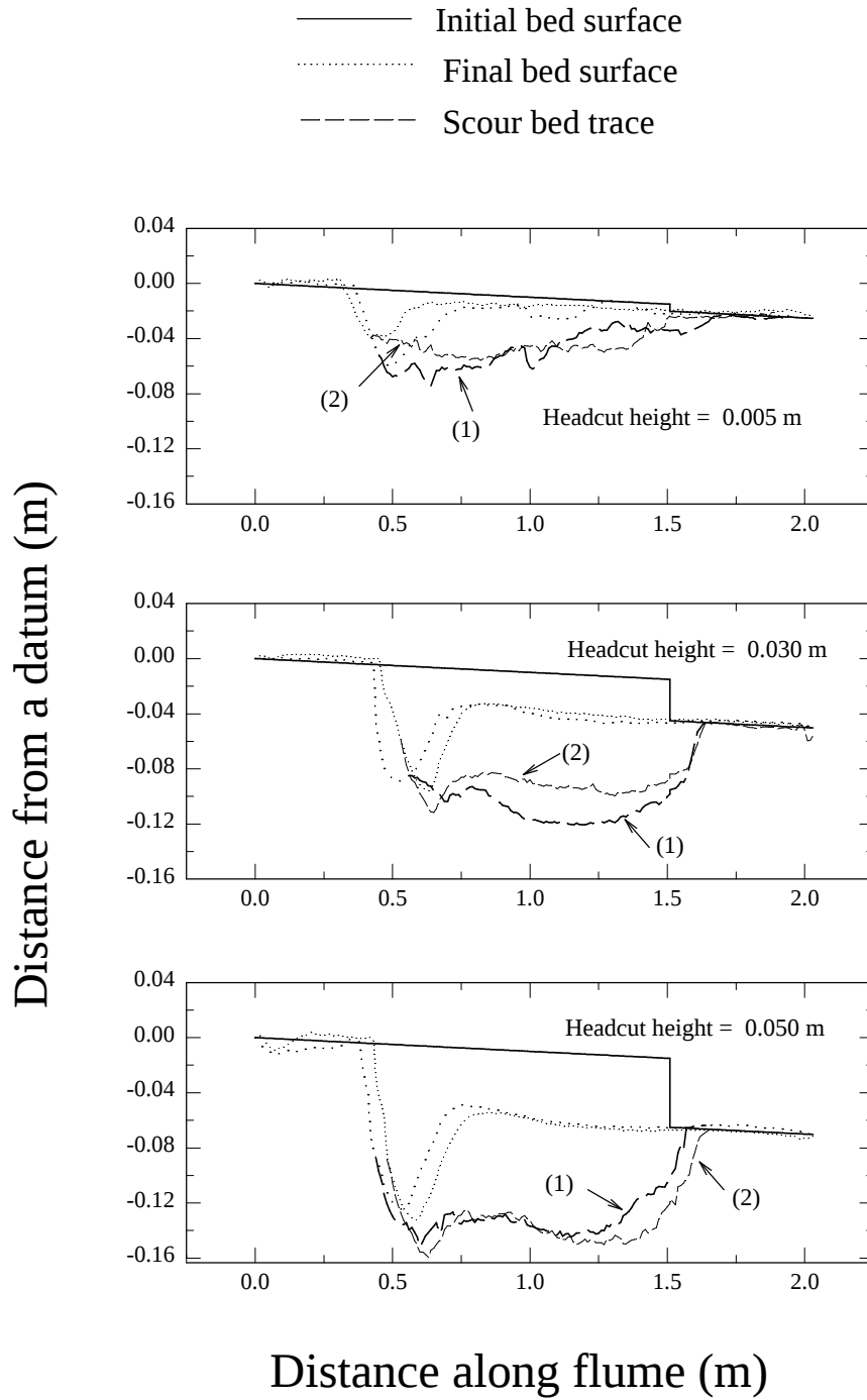
Along flume profiles of the initial and final bed surface and the trace of the scour depth for the repeated experiments. (a) 0.005(1) and 0.005(2); (b) 0.030(1) and 0.030(2); 0.050(1) and 0.050(2). Flow is from left to right.
