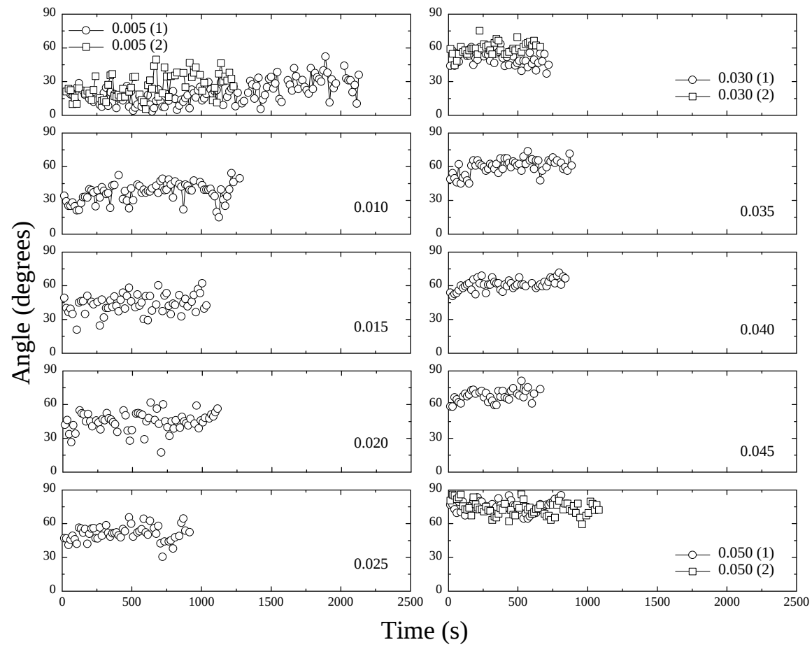
Time variation in jet angle measured at 15-s intervals.
