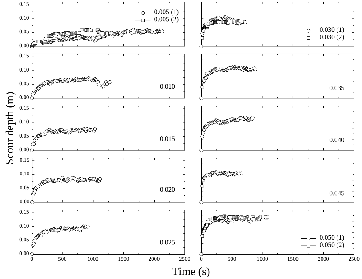
Time variation of maximum scour depth S_D measured at 15-s intervals.
