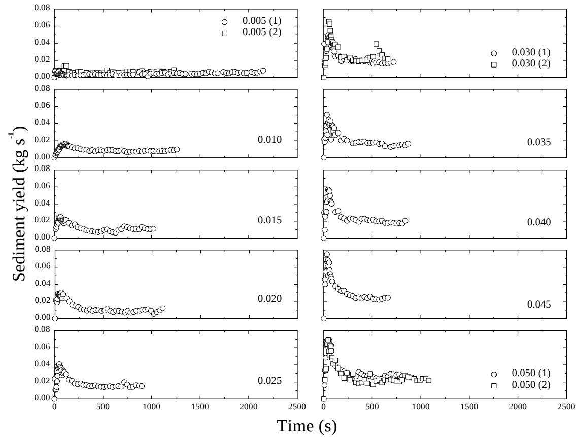
Time variation in sediment yield for all experiments. Samples were obtained as fast as possible until the headcut form and its migration rate had stabilized, and thereafter at 30-s intervals.
