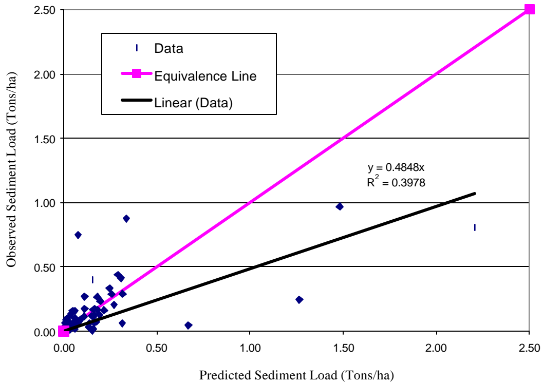
Figure 20. Comparison of observed and predicted sediment yield by event.
