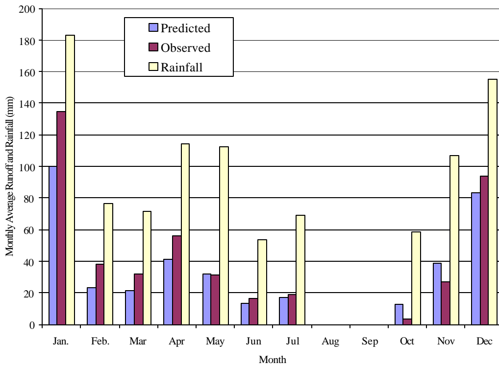
Figure 19. Comparison of monthly average predicted and observed runoff with associated rainfall.
