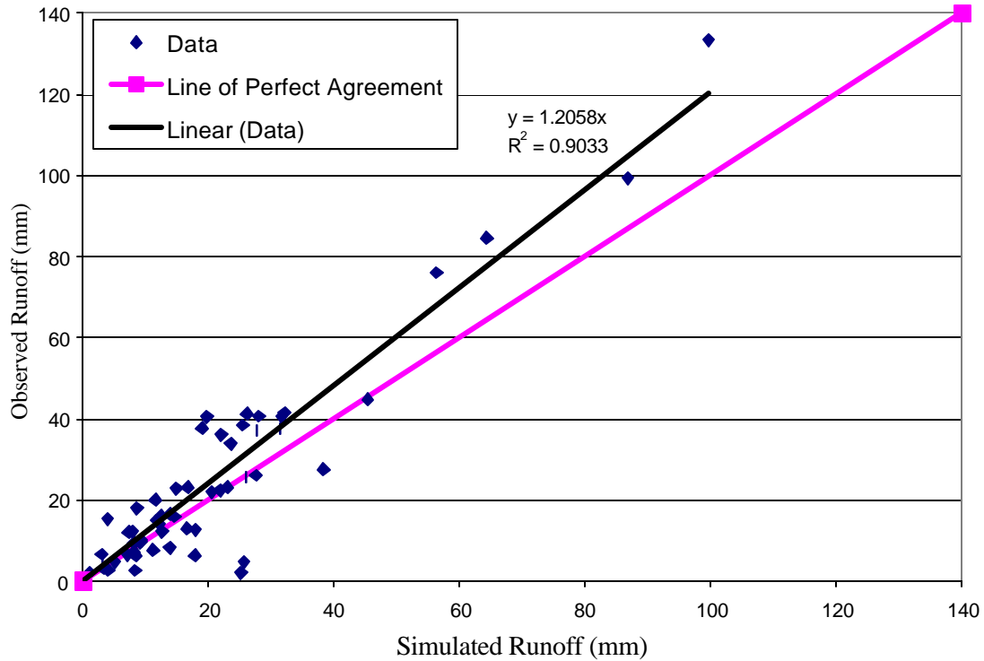
Figure 18. Comparison of observed and simulated runoff by event.
