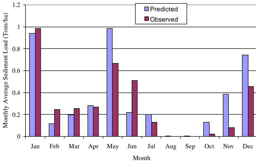
Figure 21. Comparison of predicted and observed monthly average sediment yield.
