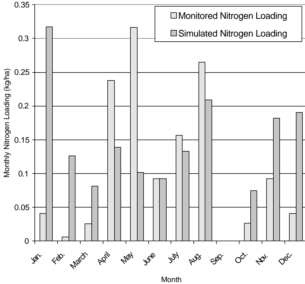
Figure 22. Comparison of monthly average predicted and observed nitrogen loading.
