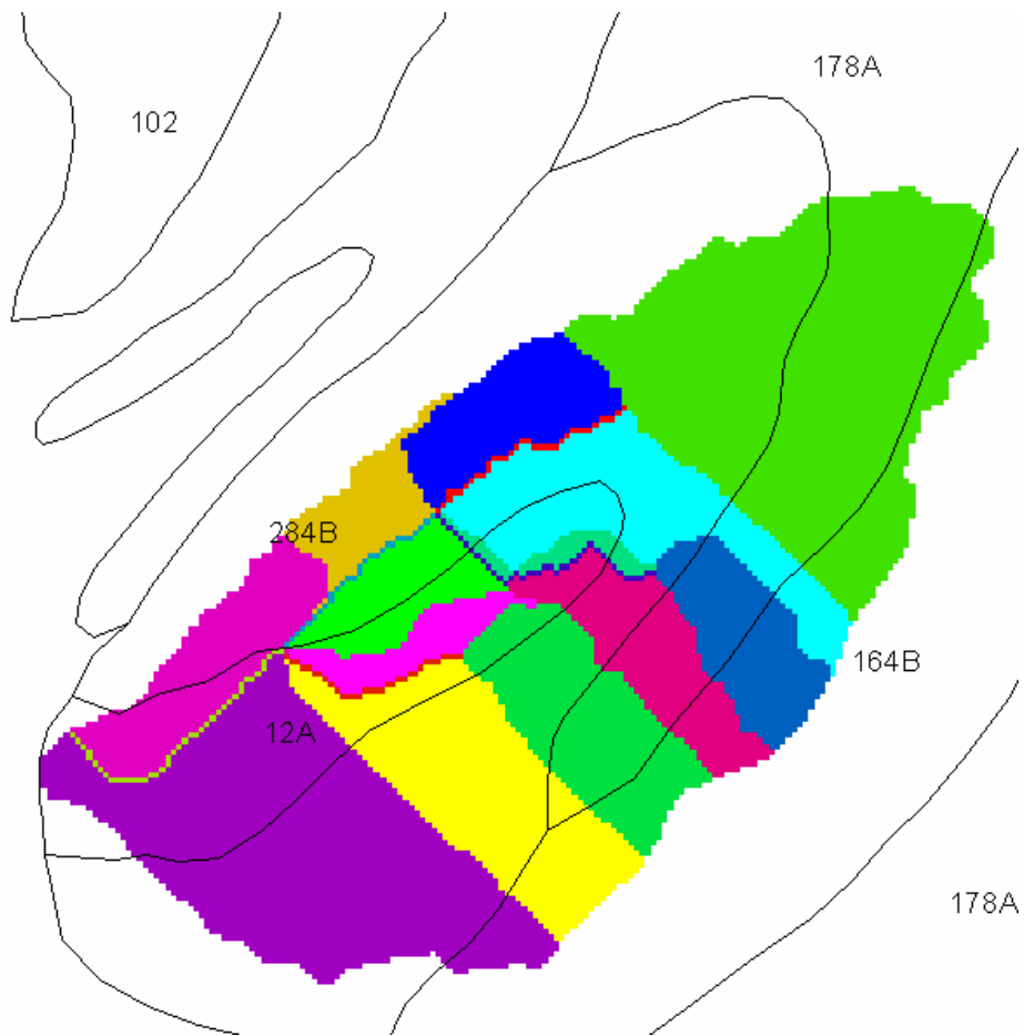
Figure 15. Overlay of soil information on the delineated watershed and subwatersheds for monitoring flume UL2
