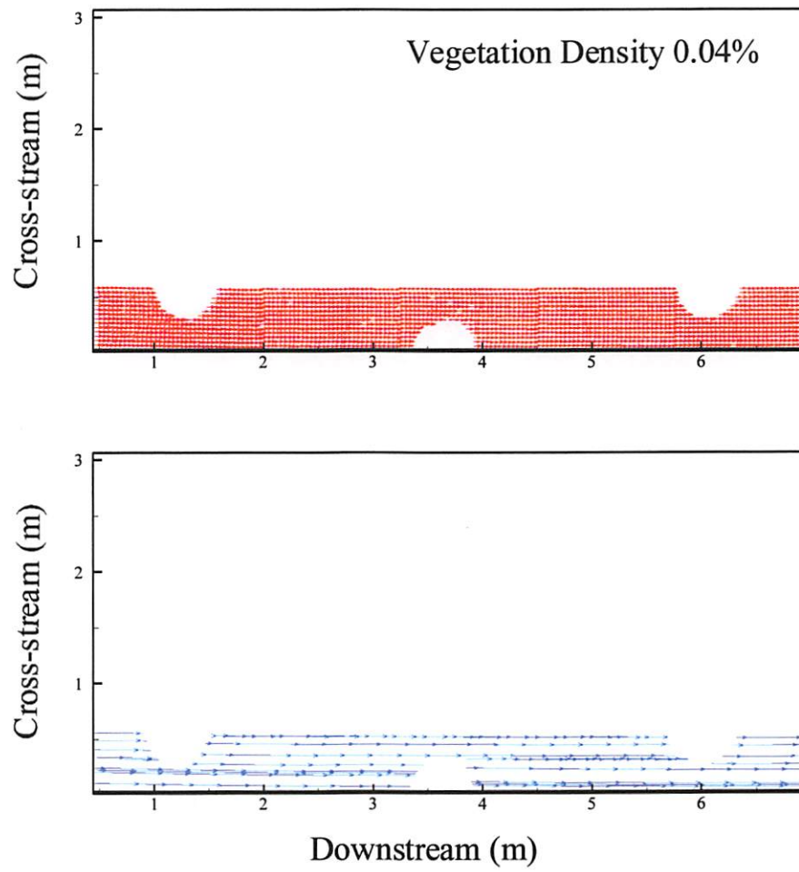
Figure 4-5. Plan view of (a) time averaged velocity vectors (b) streamlines of the flow vectors for a vegetation density of 0.04%.
