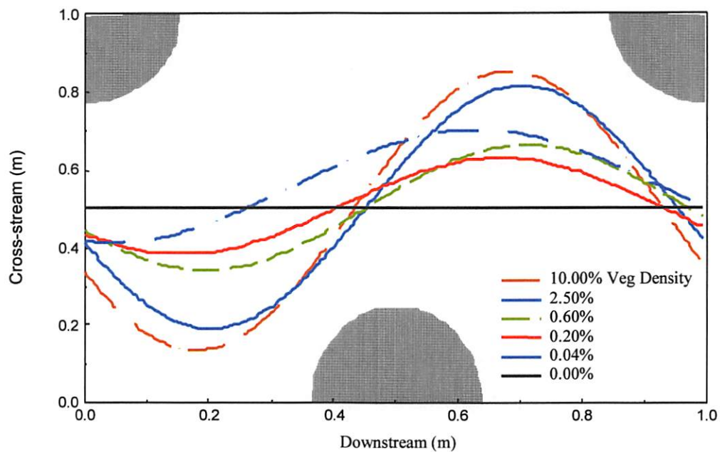
Figure 4-13. Path of maximum velocity around the vegetated zones.
