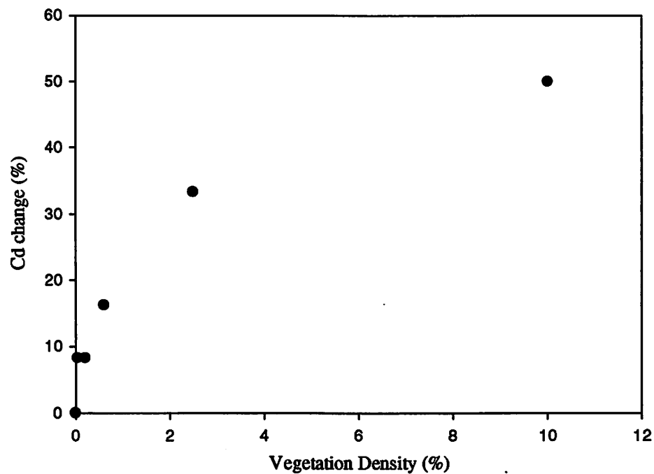
Figure 4-19. Drag coefficient change as a function of vegetation density.
