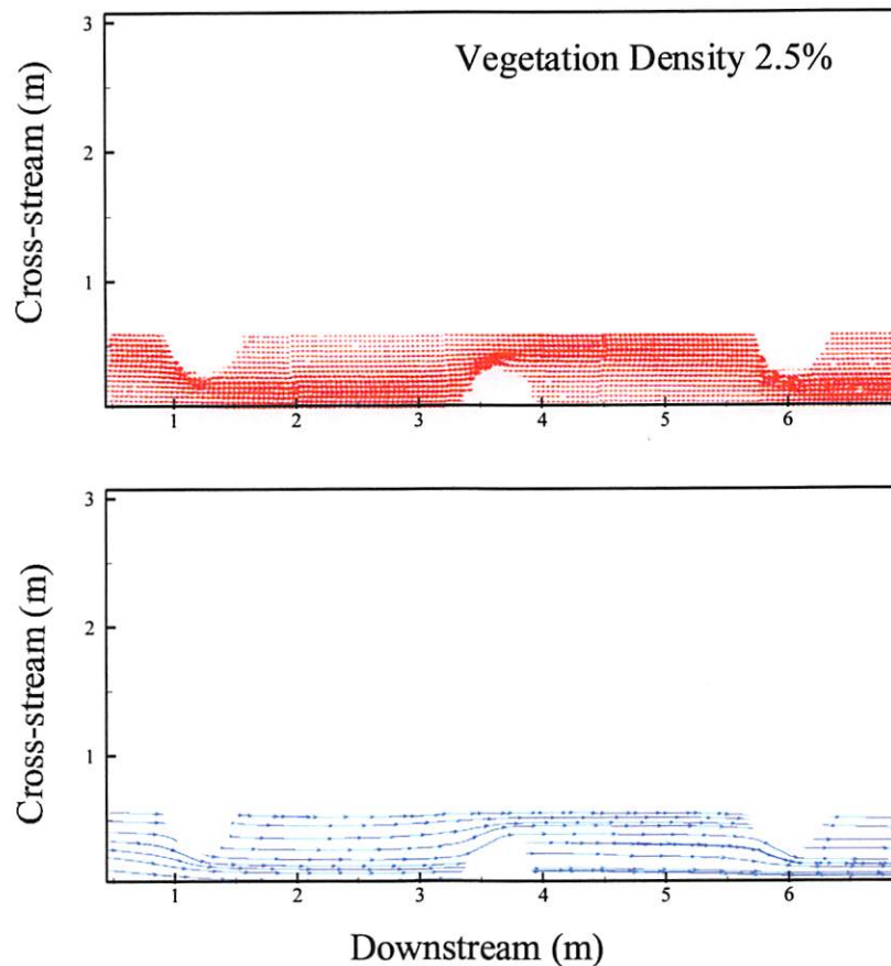
Figure 4-2. Plan view of (a) time averaged velocity vectors (b) streamlines of the flow vectors for a vegetation density of 2.5%.
