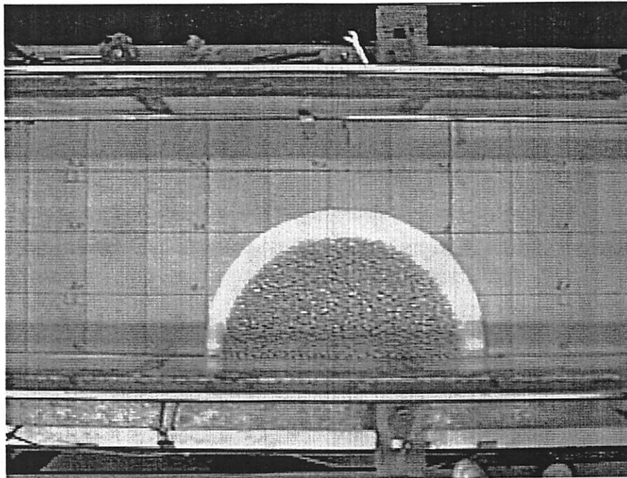
Figure 3-7. The grid scale image of the vegetated zone section.
