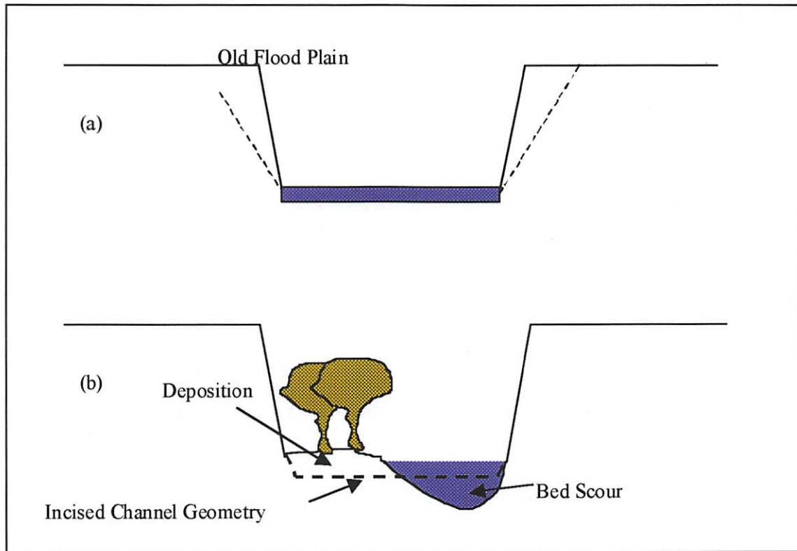
Figure 1-5. The cross-section of (a) non-vegetated incised stream with unstable bank; (b) vegetated incised stream.
