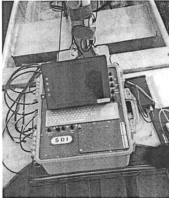
Figure 4-3. Photograph of acoustic profiling system (May 2001).
