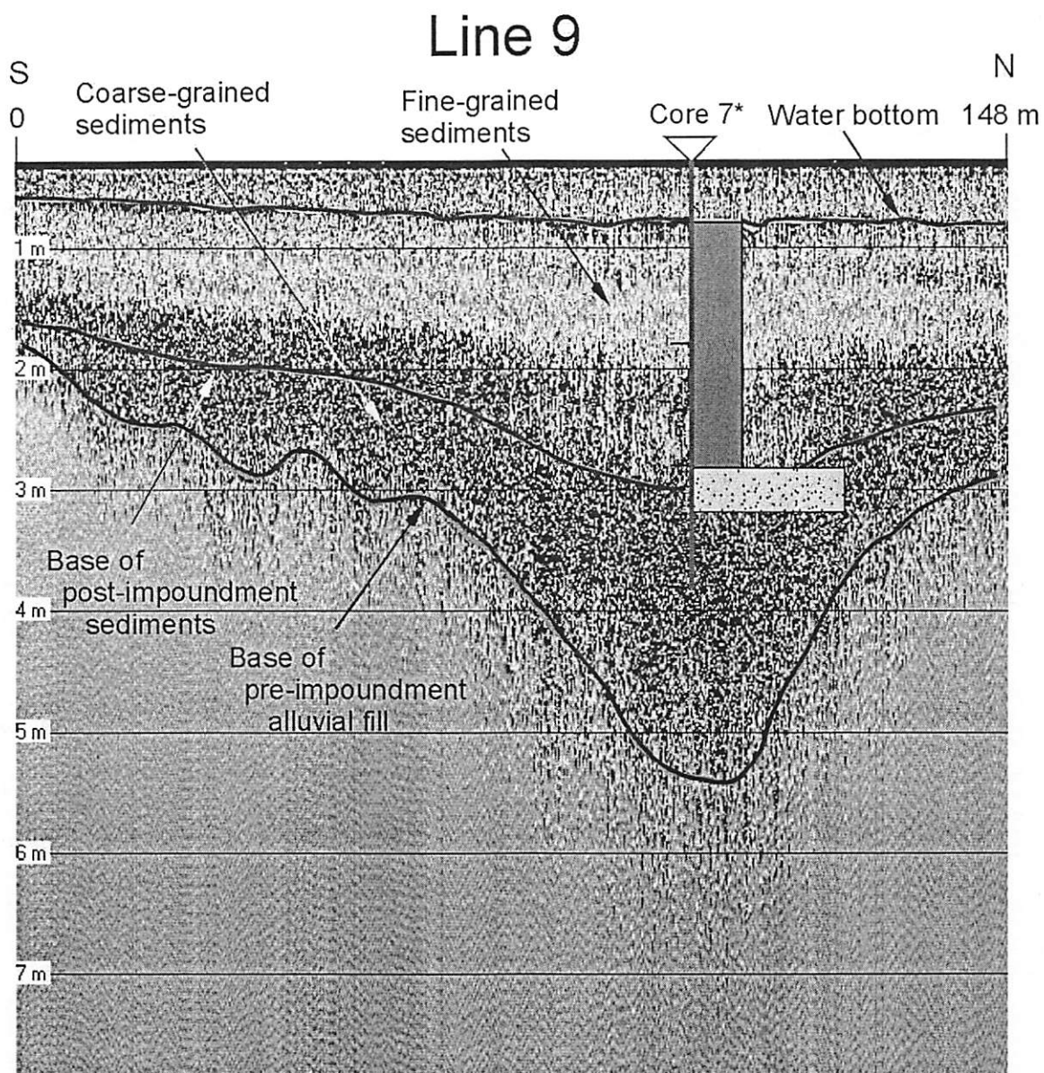
Figure 4-8. Processed Line 9 with interpretation. See Figure 4-5 for line position. The position of Core 7 from Bennett and Cooper (2001) is projected onto the line from a distance of 19 m.
