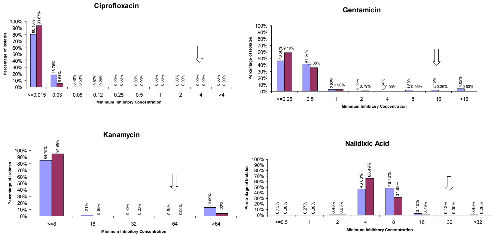
Fig. 5 Minimum Inhibitory Concentrations by Antimicrobial Agent for All Salmonella Isolates from Swine
