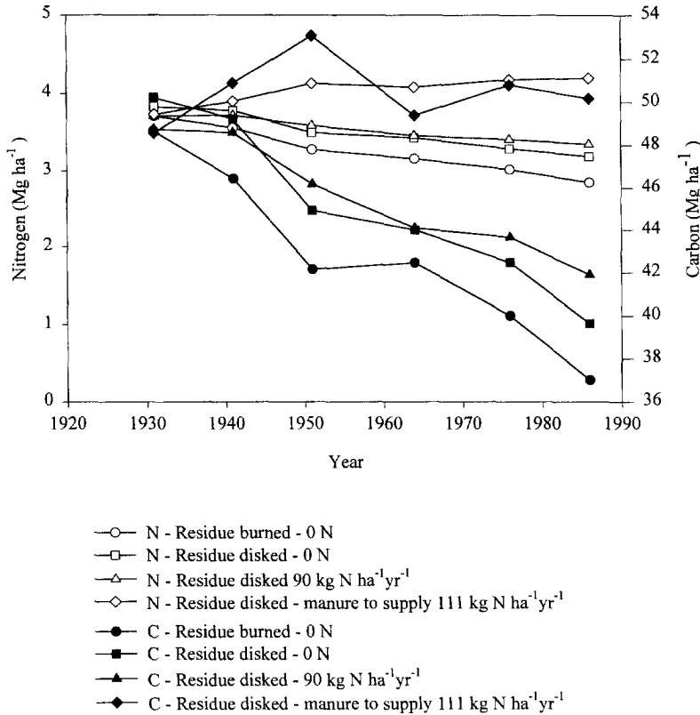
Fig. 2. Soil organic C and organic N (0 to 30 cm depth) from long-term residue management study, Pendleton, OR, USA, as affected by amendment and residue management (from Duff et al., 1995).
