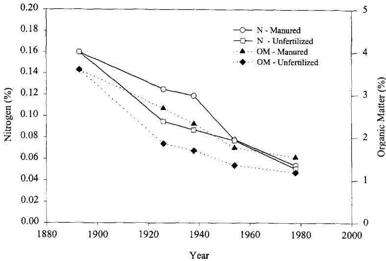
Fig. 1. Nitrogen and organic matter content of surface soil from manured and unfertilized wheat plots in the Magruder Plots, OK, USA (from Webb et al., 1980).
