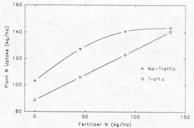
Fig. 6. Effect of traffic on total plant N uptake at harvest in 1991.
