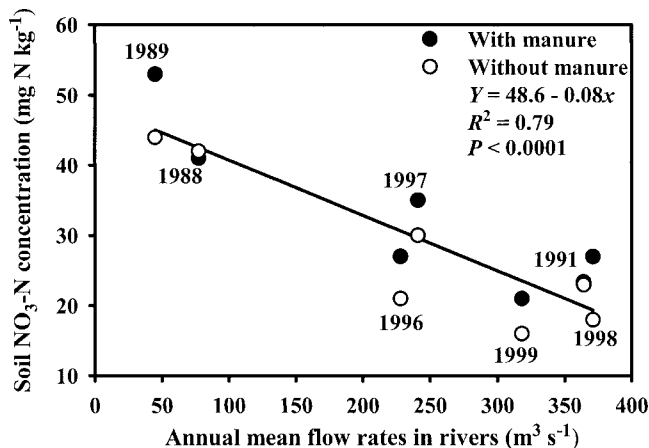
Fig. 5. Relationship between annual means for soil NO 3 -N concentrations in early June and annual means for flow in the Des Moines and Iowa Rivers.
