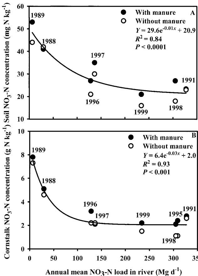
Fig. 7. Relationships between annual mean NO 3 -N loads in the Iowa River at Wapello and annual means for (A) soil NO 3 -N concentrations in late spring and (B) cornstalk NO 3 -N concentrations at the end of the growing season.
