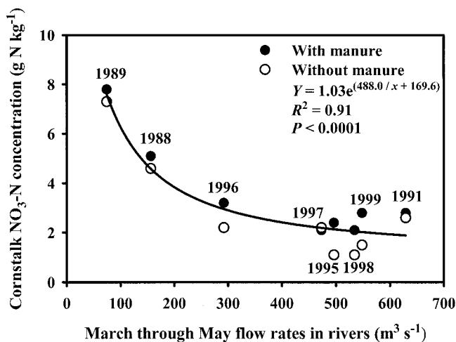
Fig. 6. Relationship between early-season water flows in the Des Moines and Iowa Rivers and annual means of cornstalk NO 3 -N concentrations measured at the end of the season.
