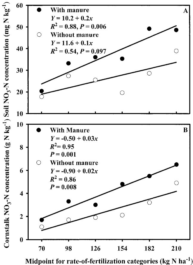
Fig. 8. Mean (A) soil and (B) cornstalk NO 3 -N concentrations for six rate-of-N-fertilization categories for soils with and without animal manure.
