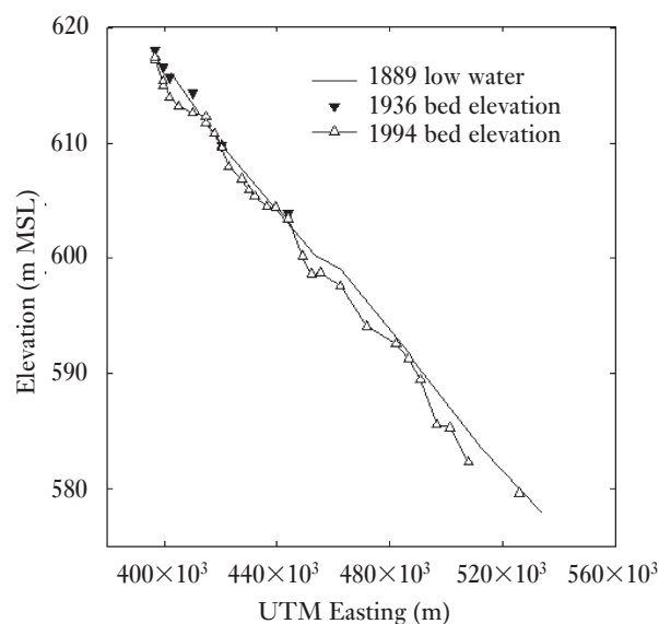
Figure 2 Elevation of the bed of the Missouri River downstream from Fort Peck Dam. The 1889 elevations are based on a low-water profile published by the US Army Corps of Engineers (1933). The dam was closed in 1937. The 1936 and 1994 mean bed elevations are from Wei (1997).
