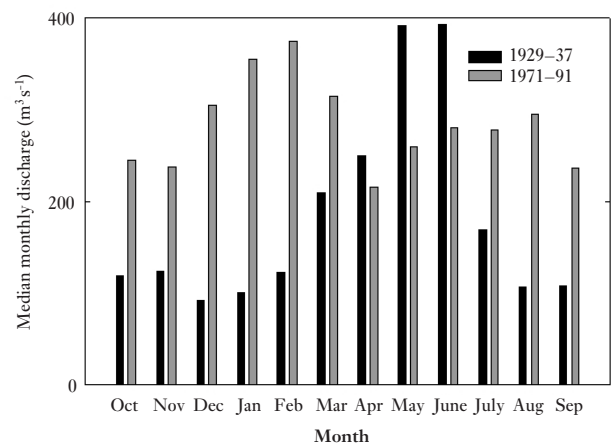
Figure 4 Median value of mean daily discharge in ( \text{m}^3 \text{s}^{-1} ) by month for Missouri River at Wolf Point, Montana. Time periods are selected intervals before and after closure of Fort Peck Dam.
