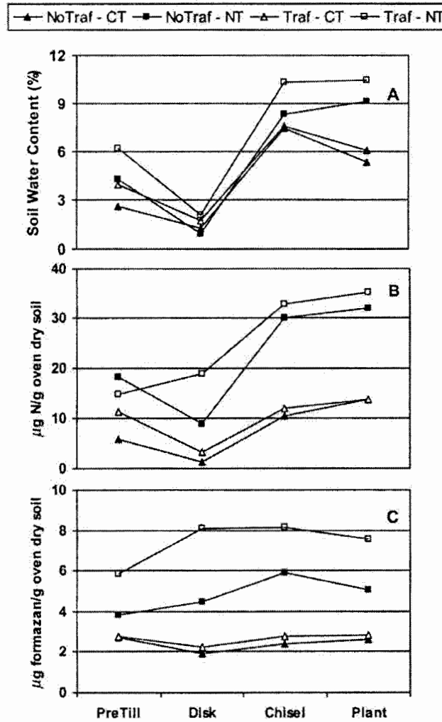
Figure 1. Interactive effects of traffic (NoTraf = no traffic; Traf = traffic) and tillage system (CT = conventional tillage; NT = no tillage) on soil water content (A), soil microbial biomass nitrogen (B), and dehydrogenase (C). Sampling periods on the X-axis are prior to spring tillage (PreTill), following disking (Disk), following chisel plowing (Chisel), and following cultivator/planter operation (Plant).
