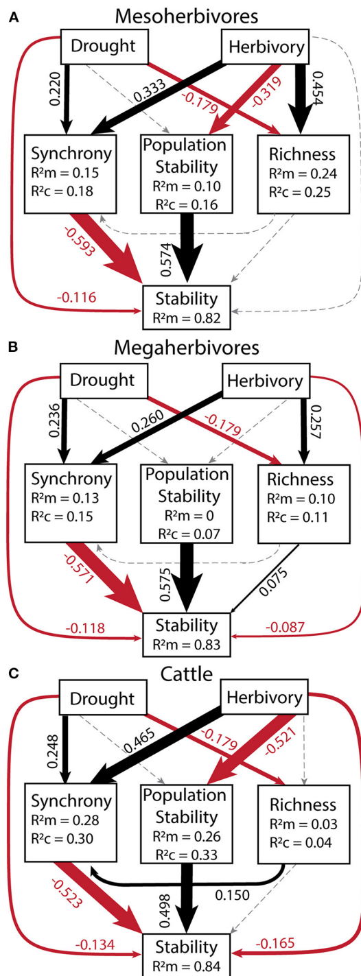
FIGURE 6 | Structural equation models for each herbivore group: mesoherbivores (A), megaherbivores (B), and cattle (C) to determine the relative strength of direct vs. indirect effects of drought and herbivory. All variables in the model were calculated over a 10-year moving window in order to compare to the corresponding drought score of each time window. Goodness of Fit values were: for mesoherbivores C = 4.00 , p = 0.406 , df = 4 (A), for megaherbivores C = 8.86 , p = 0.065 , df = 4 (B), and for cattle C = 13.79 , p = 0.008 , df = 4 (C). Values next to arrows (direct effects) are scale standardized estimates of coefficients and arrow width is scaled to their (Continued)
