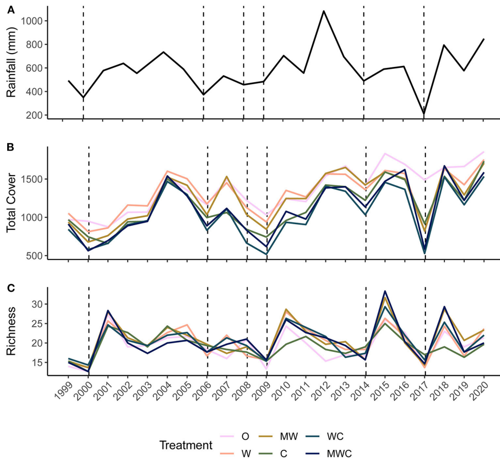
FIGURE 2 | Precipitation (mm) calculated over the 12-months before the annual June sampling period (A) , mean total cover (B) and species richness (C) at each sampling point (annually in June) from 1999–2020 colored by herbivore treatment. Herbivore treatments (ordered by total herbivore biomass) are: O, No herbivores; W, Wild mesoherbivores; MW, Wild mega-herbivores and wild mesoherbivores; C, Cattle; WC, Wild mesoherbivores and cattle; MWC, Wild mega-herbivores, wild mesoherbivores, and cattle. Dashed lines indicate low rainfall (<the 25th percentile, defined here as a drought) in the 12 months preceding the sampling point.
