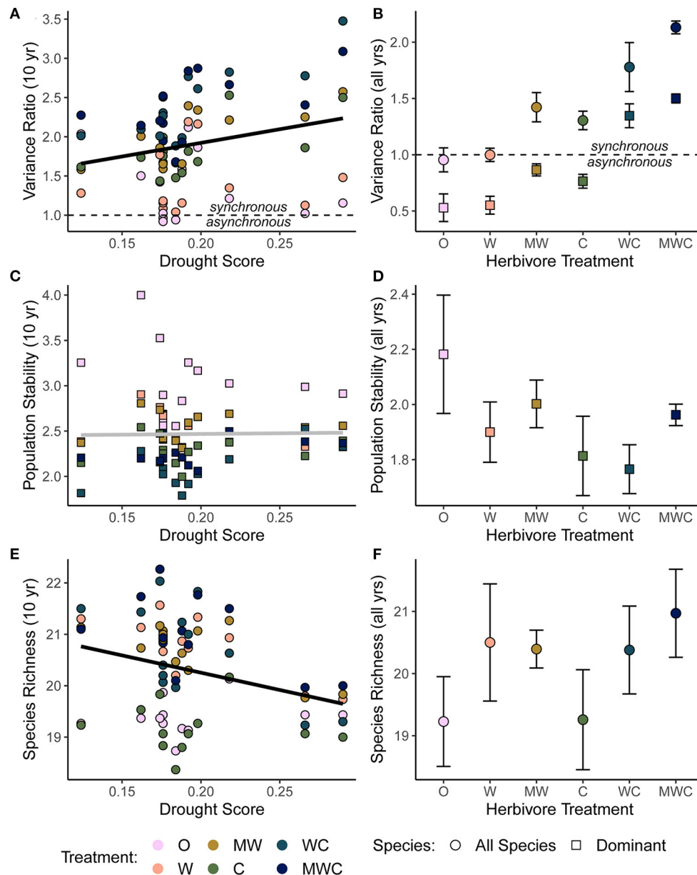
FIGURE 4 | The relationship between the variance ratio (A), dominant species population stability (C), species richness (E) and drought, all calculated over a 10-year moving window in order to compare to the corresponding drought score of each time window. The effects of herbivore treatment on the variance ratio (B), dominant species population stability (D), and species richness (F) calculated as an average over the full timeseries. A variance ratio less than one indicates asynchronous dynamics, and greater than one indicates synchronous dynamics. Shape indicates whether the biotic mechanism is calculated using all species in the community (circles) or only the five dominant species (squares). Bars are one standard error. Black regression lines in (A,E) are plotted when the predictor was included in the top model and the gray regression line in (C) indicates that this predictor did not have an effect. Figures are based on raw data, but statistical models include random effects to account for spatial and temporal autocorrelation. See Tables 2, 3 for model details. Herbivore treatments (ordered by total herbivore biomass) are: O, No herbivores; W, Wild mesoherbivores; MW, Wild megaherbivores and wild mesoherbivores; C, Cattle; WC, Wild mesoherbivores and cattle; MWC, Wild megaherbivores, wild mesoherbivores, and cattle.
