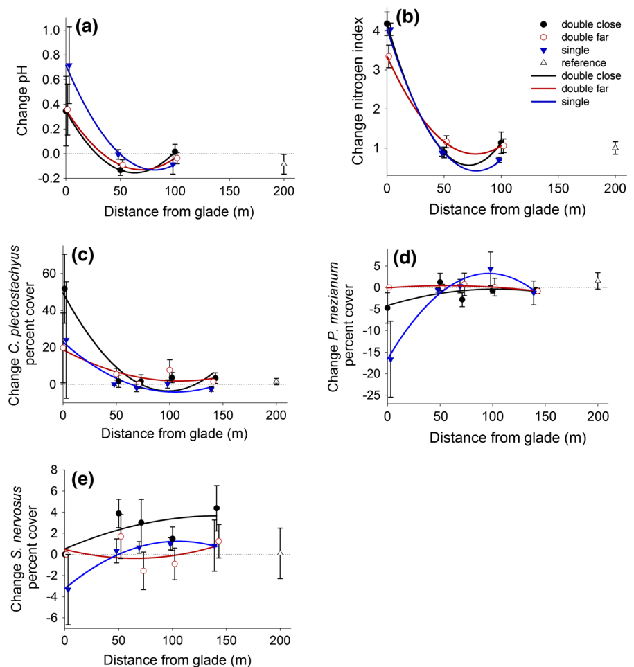
Fig. 2 Glade density treatment effects on soils, forage quality and the understory plant community. a Soil pH, b foliar nitrogen content, c C. plectostachyus cover, d P. meizianum cover, and e S. nervosus cover. Points (jittered) represent average subplot-specific changes from baseline to 18 months (for soils and forage) or 32 months (for understory plants) \pm 1 SE. Lines represent simple quadratic functions fit to the raw data
