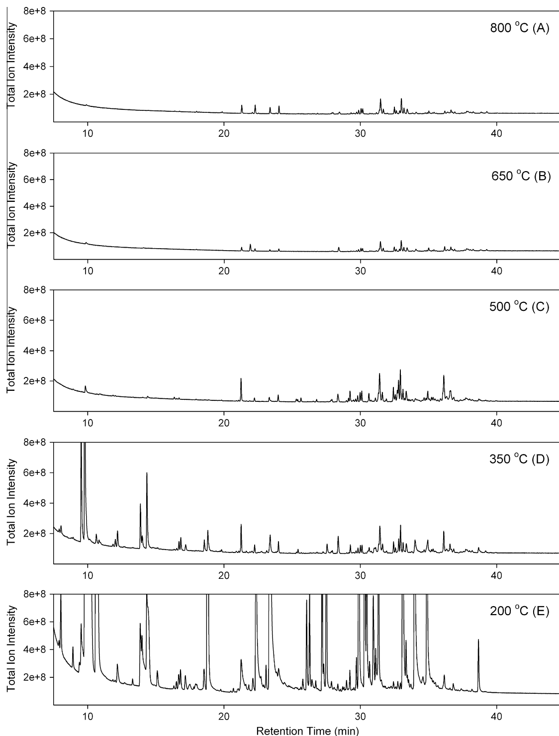
Fig. 3. Total ion chromatograms for the analysis of cottonseed hull biochar pyrolyzed at (A) 800, (B) 650, (C) 500, (D) 350, and (E) 200 °C for 4 h under 1600 mL min -1 N 2 flow. All chromatograms are scaled equally.
