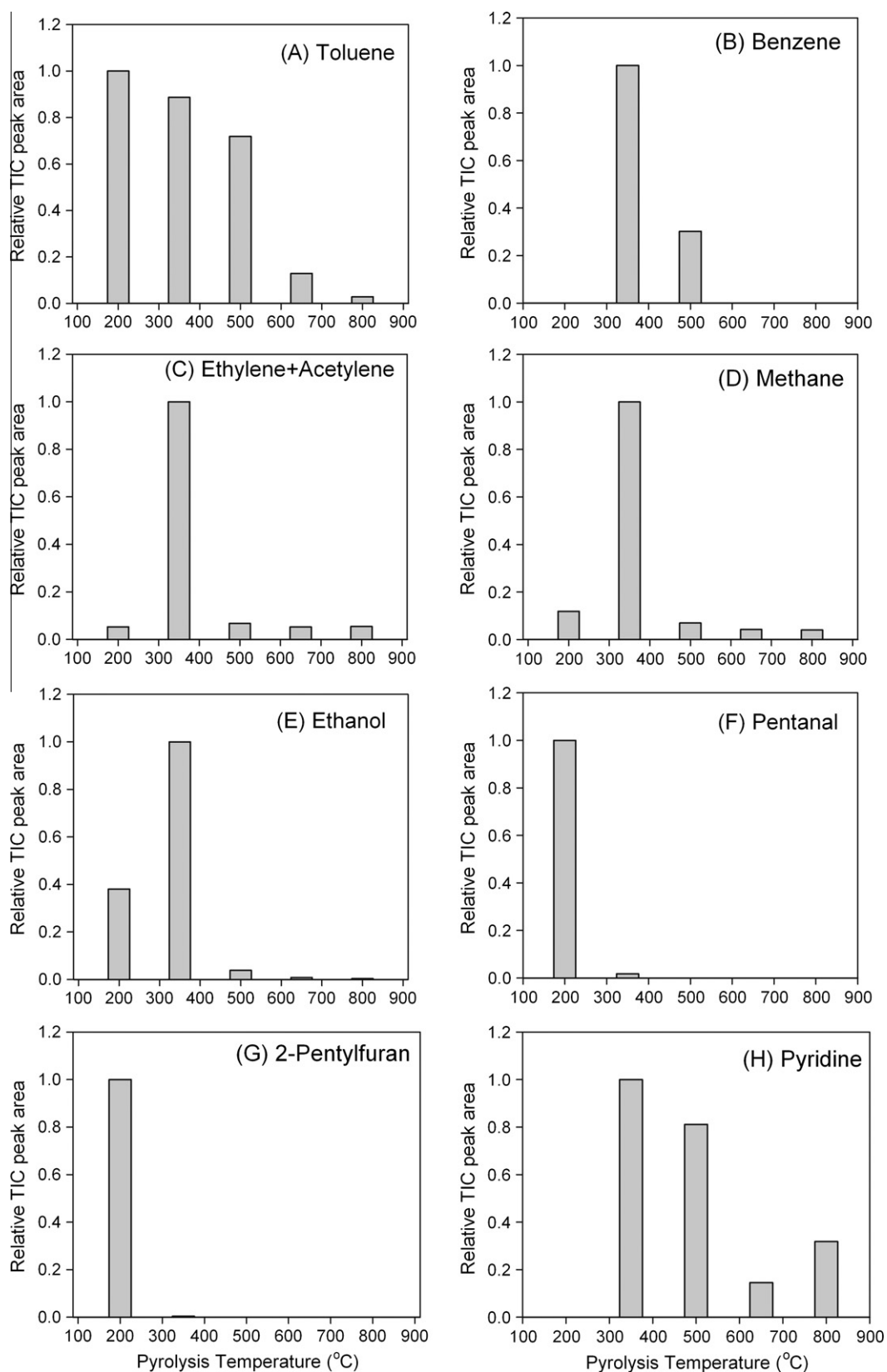
Fig. 4. Illustration of trends in relative peak areas for (A) toluene, (B) benzene, (C) ethylene-acetylene, (D) methane, (E) ethanol, (F) pentanal, (G) 2-pentylfuran, and (H) pyridine detected in cottonseed hull biochars as a function of pyrolysis temperature.
