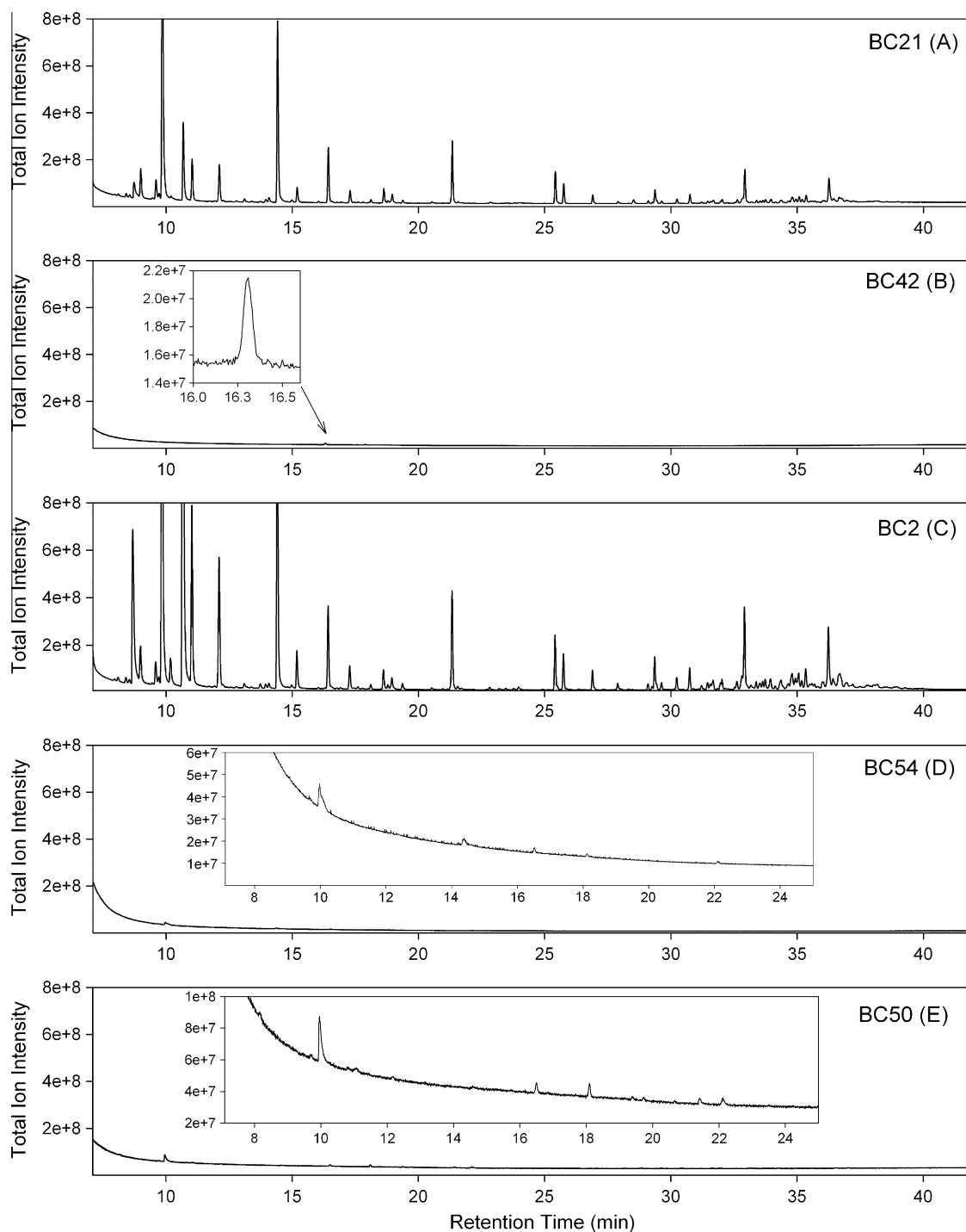
Fig. 1. Images of the total ion chromatograms from the thermal desorption GC/MS analysis of five different oak hardwood biochars: (A) Slow pyrolysis (BC21), (B) Slow pyrolysis (BC42), (C) Fast pyrolysis (BC2), (D) Gasifier (BC54), and (E) Tradition soil mound kiln (BC50) production methods. All chromatograms are scaled equally, with the inset chromatograms showing the rescaled chromatogram. All pyrolysis techniques had nearly equivalent production temperatures.
