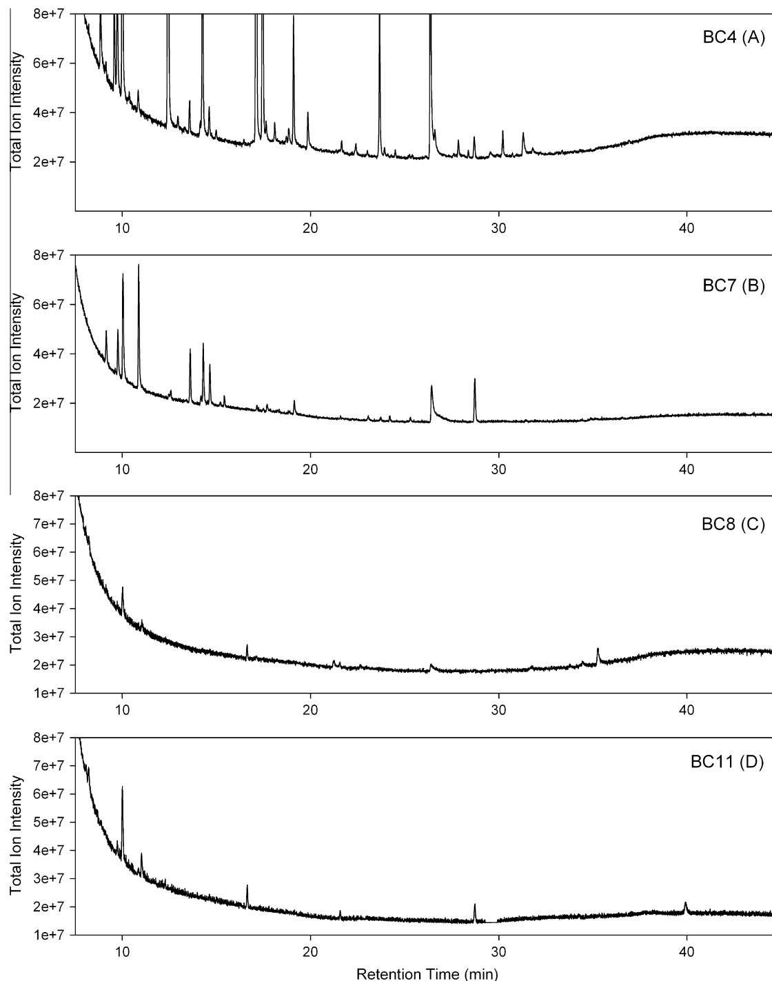
Fig. 2. Illustrations of the headspace thermal desorption GC/MS total ion chromatograms for corn stover biochar produced by four different slow pyrolysis units: (A) BC4, (B) BC7, (C) BC8, and (D) BC11. All chromatograms are scaled equally and had nearly equivalent production temperatures.
