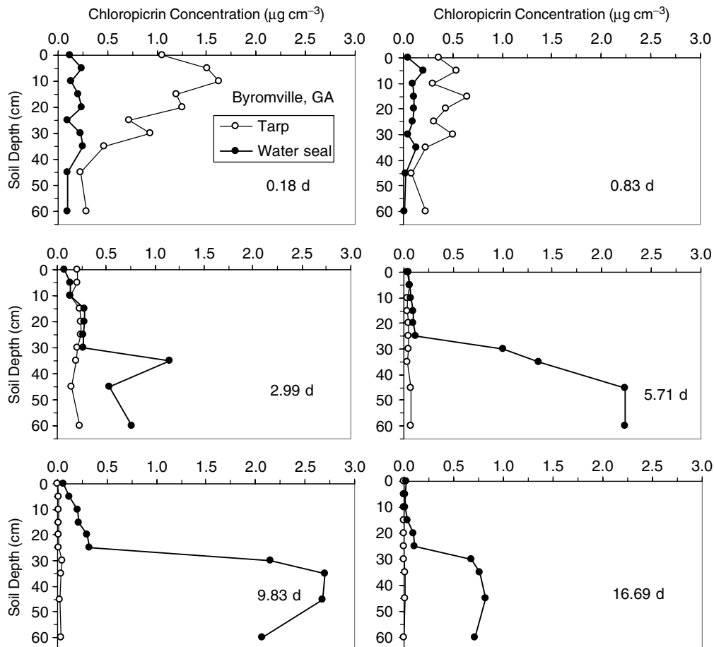
Figure 6. Average concentrations of chloropicrin in soil air at 0.18, 0.83, 2.99, 5.71, 9.83 and 16.69 days (d) after injection at Byromville, GA on 9 September 2003.
