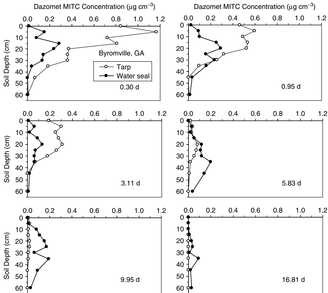
Figure 2. Average concentrations of methyl isothiocyanate (MITC) in soil air at 0.30, 0.95, 3.11, 5.83, 9.95 and 16.81 days (d) after application of dazomet at Byromville, GA on 9 September 2003.
