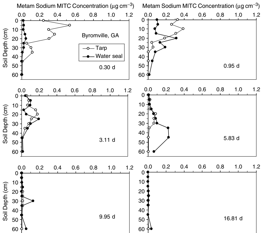
Figure 4. Average concentrations of methyl isothiocyanate (MITC) in soil air at 0.30, 0.95, 3.11, 5.83, 9.95 and 16.81 days (d) after application of metam-sodium at Byromville, GA on 9 September 2003.
