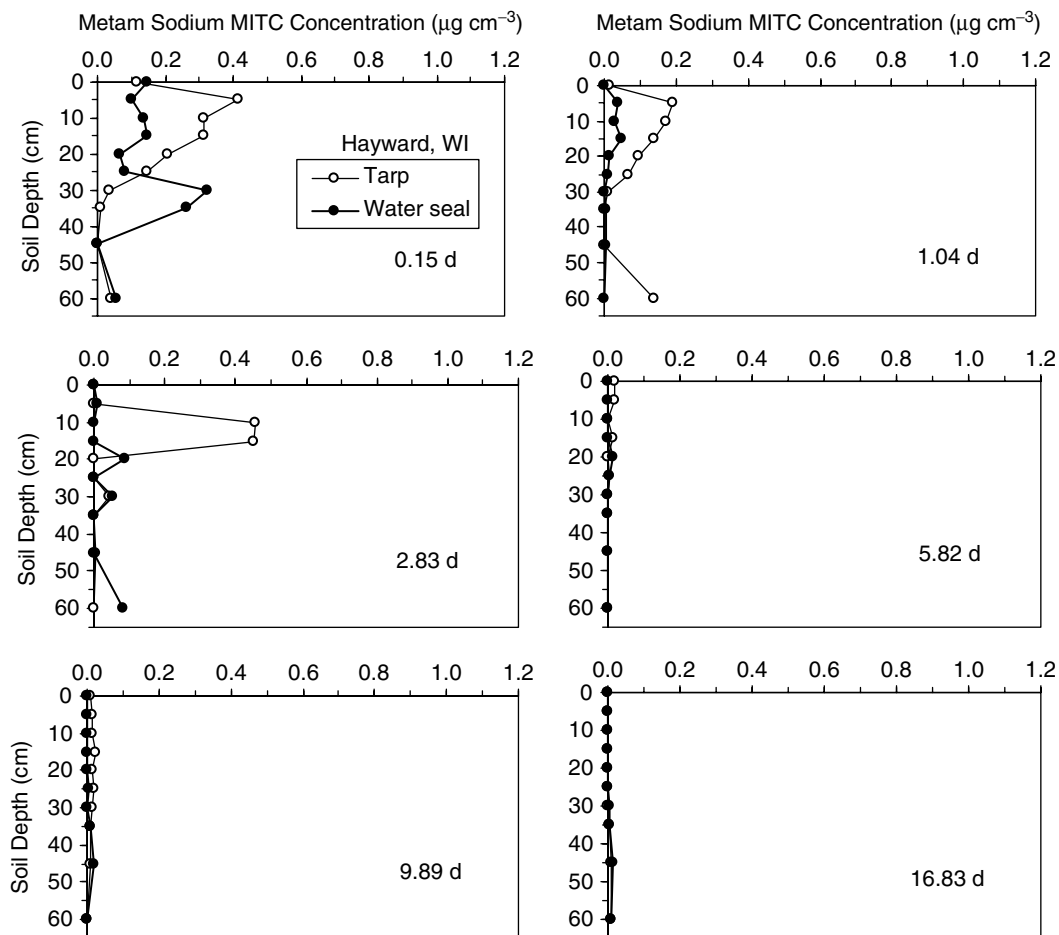
Figure 3. Average concentrations of methyl isothiocyanate (MITC) in soil air at 0.15, 1.04, 2.83, 5.82, 9.89 and 16.83 days (d) after application of metam-sodium at Hayward, WI on 6 August 2002.
