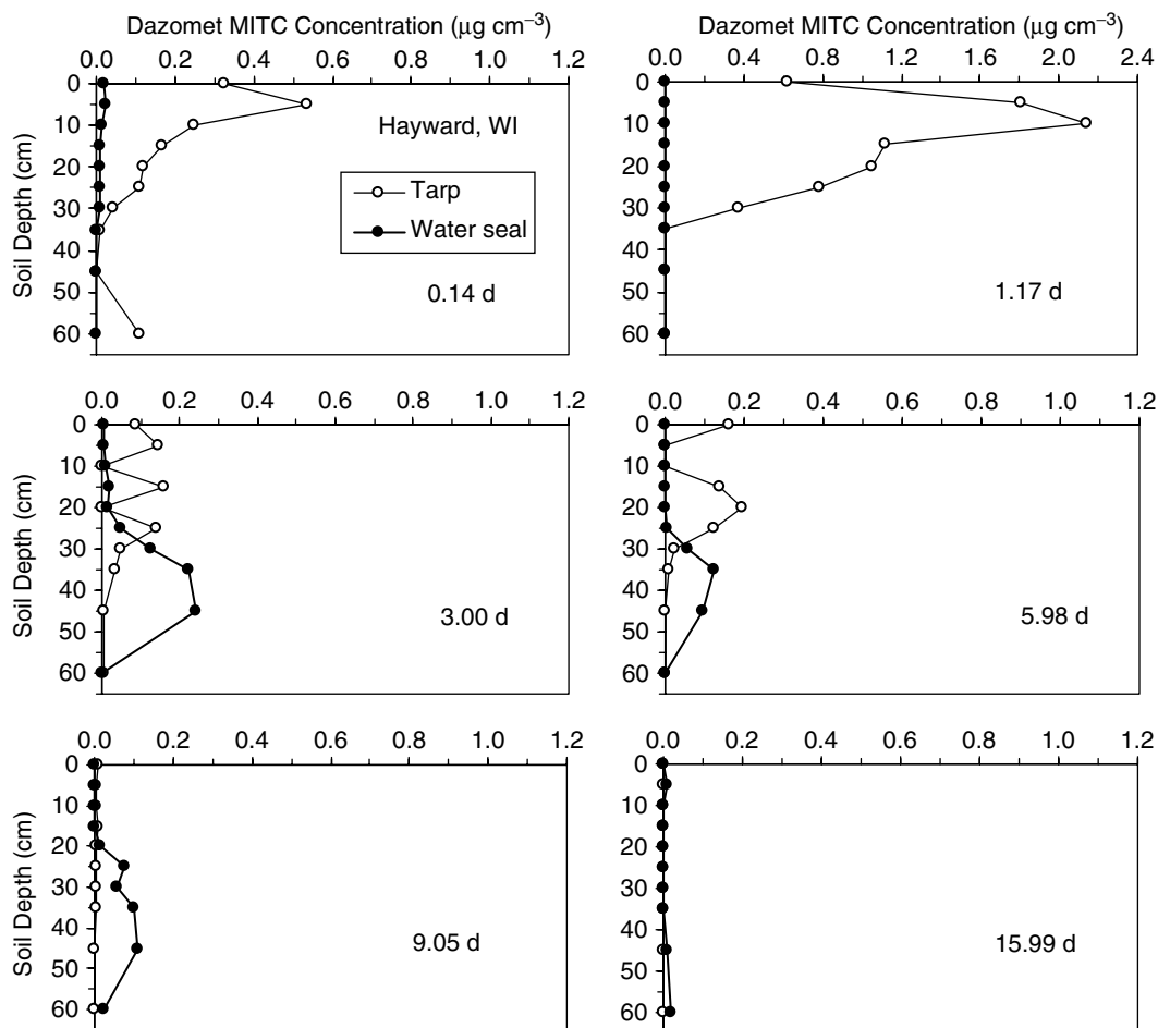
Figure 1. Average concentrations of methyl isothiocyanate (MITC) in soil air at 0.14, 1.17, 3.00, 5.98, 9.05 and 15.99 days (d) after application of dazomet at Hayward, WI on 7 August 2002.
