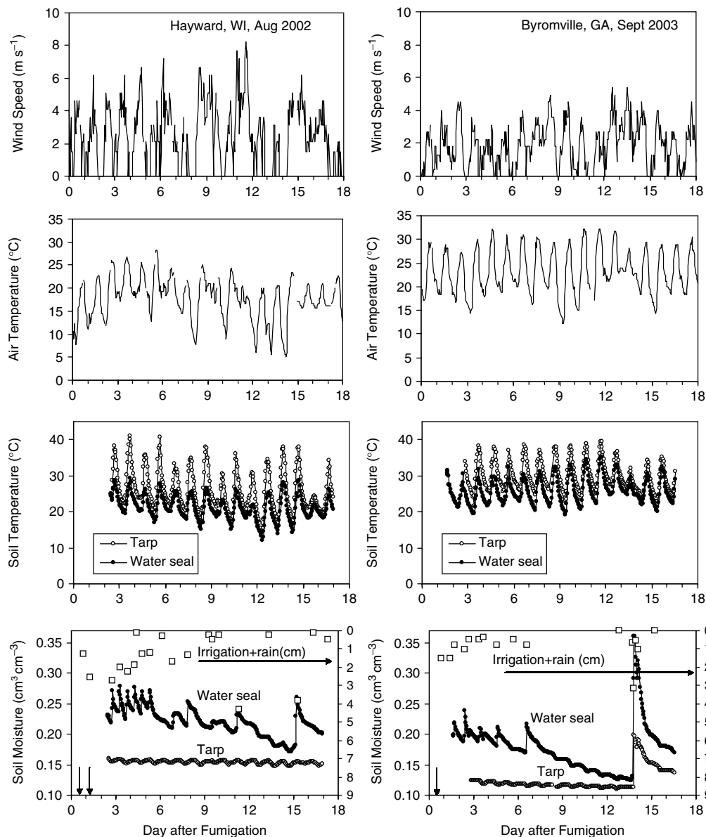
Figure 7. Wind speed, air temperature, soil temperature and soil moisture during the fumigation experiments at Hayward, WI and Byromville, GA. Day after fumigation was referenced to 12:00 on 6 August 2002 and 12:00 on 9 September 2003 for the Hayward and Byromville experiments respectively. The first arrow in the lower left graph points to the time (14:10 on 6 August) of metam-sodium and chloropicrin application and the second arrow to the time (10:45 on 7 August) of dazomet application at Hayward, WI. The arrow in the lower right graph indicates the time (11:30 on 9 September) of dazomet and metam-sodium application at Byromville, GA, where chloropicrin was injected 4 h later. Soil temperature and moisture data were for the 10 cm depth measurement from tarp and water seal treatments respectively. Open squares represent the sum of irrigation and rain (cm).
