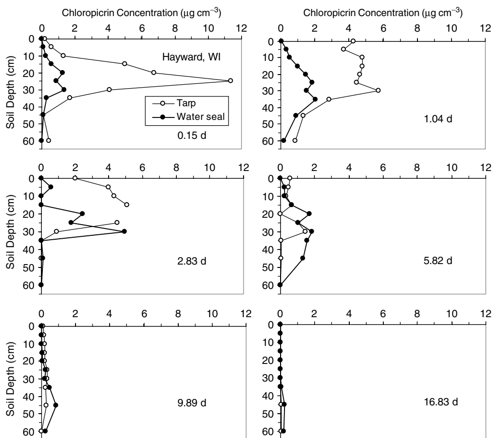
Figure 5. Average concentrations of chloropicrin in soil air at 0.15, 1.04, 2.83, 5.82, 9.89 and 16.83 days (d) after injection at Hayward, WI on 6 August 2002.
