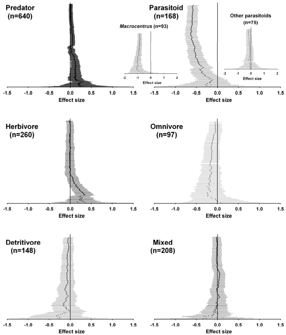
Fig. S3-1. Cumulative effect size of all Bt crops pooled when compared to non-Bt controls receiving no insecticides.
