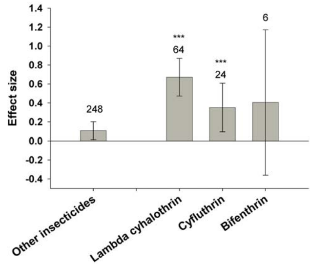
Figure 3. Effects of Bt maize vs. control fields treated with a pyrethroid insecticide on predatory arthropods. Bars denote the 95% confidence intervals, asterisks denote significant heterogeneity in the observed effect sizes among the studies (* <0.05, ** <0.01, *** <0.001), and Arabic numbers indicate the number of observations included for each functional group. doi:10.1371/journal.pone.0002118.g003
