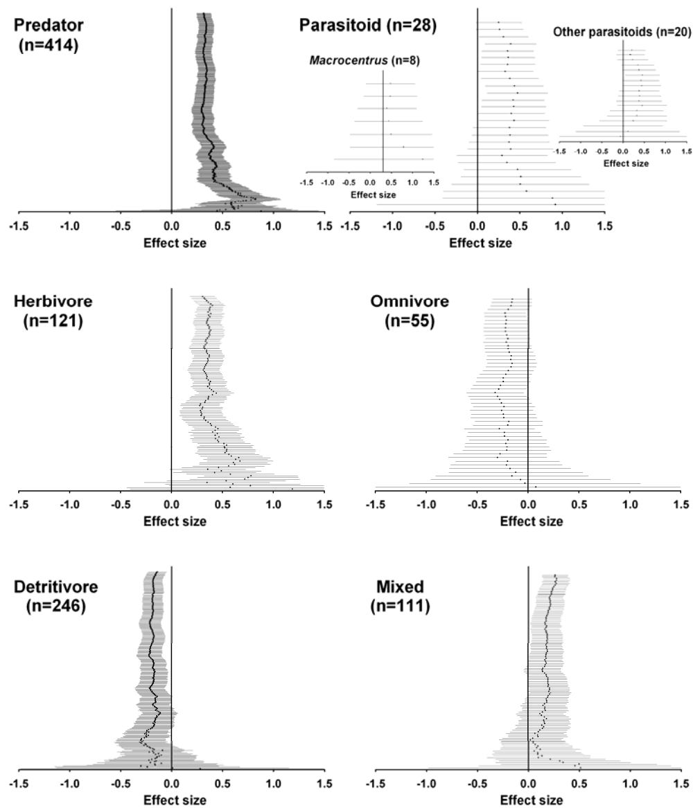
Fig. S3-2. Cumulative effect size of all Bt crops pooled when compared to non-Bt controls treated with insecticides.
