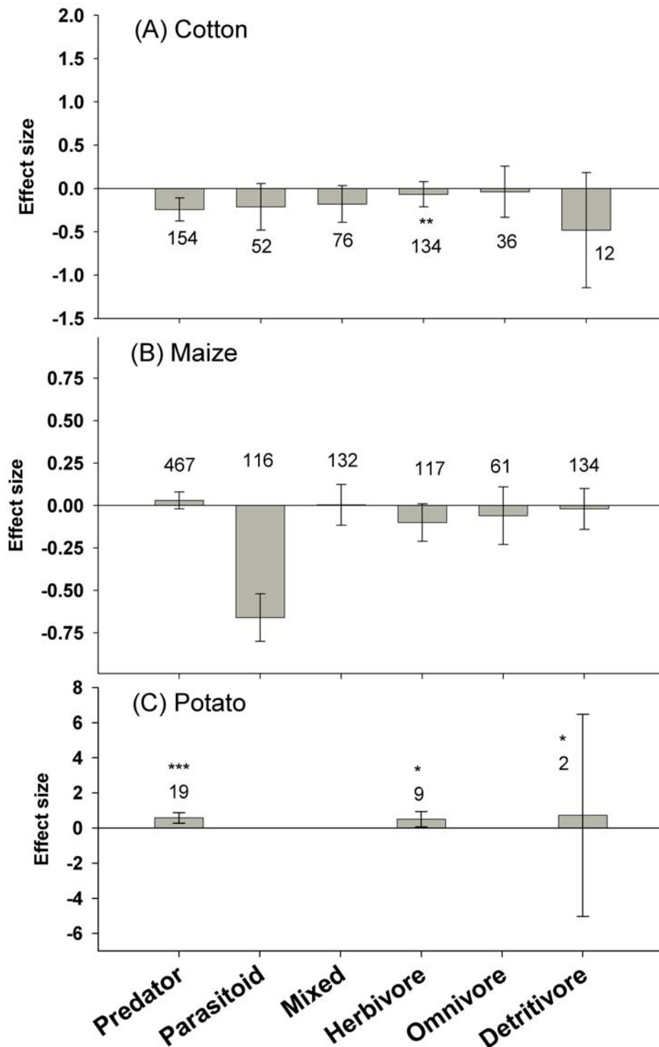
Figure 1. The effect of Bt crops on non-target functional guilds compared to unsprayed, non-Bt control fields. Bars denote the 95% confidence intervals, asterisks denote significant heterogeneity in the observed effect sizes among the comparisons (* < 0.05, ** < 0.01, *** < 0.001), and Arabic numbers indicate the number of observations included for each functional group. doi:10.1371/journal.pone.0002118.g001
