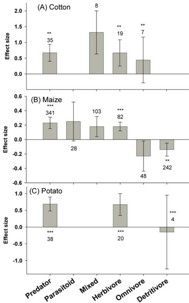
Figure 2. The effect of Bt crops on non-target functional guilds compared to insecticide-treated, non-Bt control fields. Bars denote the 95% confidence intervals, asterisks denote significant heterogeneity in the observed effect sizes among the studies (* <0.05, ** <0.01, *** <0.001), and Arabic numbers indicate the number of observations included for each functional group. doi:10.1371/journal.pone.0002118.g002
