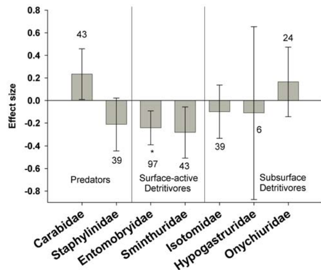
Figure 4. Effect of Bt crops vs. insecticide-treated, non-Bt control fields on soil-inhabiting predators and detritivores. Bars denote the 95% confidence intervals, asterisks denote significant heterogeneity in the observed effect sizes among the studies (* <0.05, ** <0.01, *** <0.001), and Arabic numbers indicate the number of observations included for each functional group. doi:10.1371/journal.pone.0002118.g004
