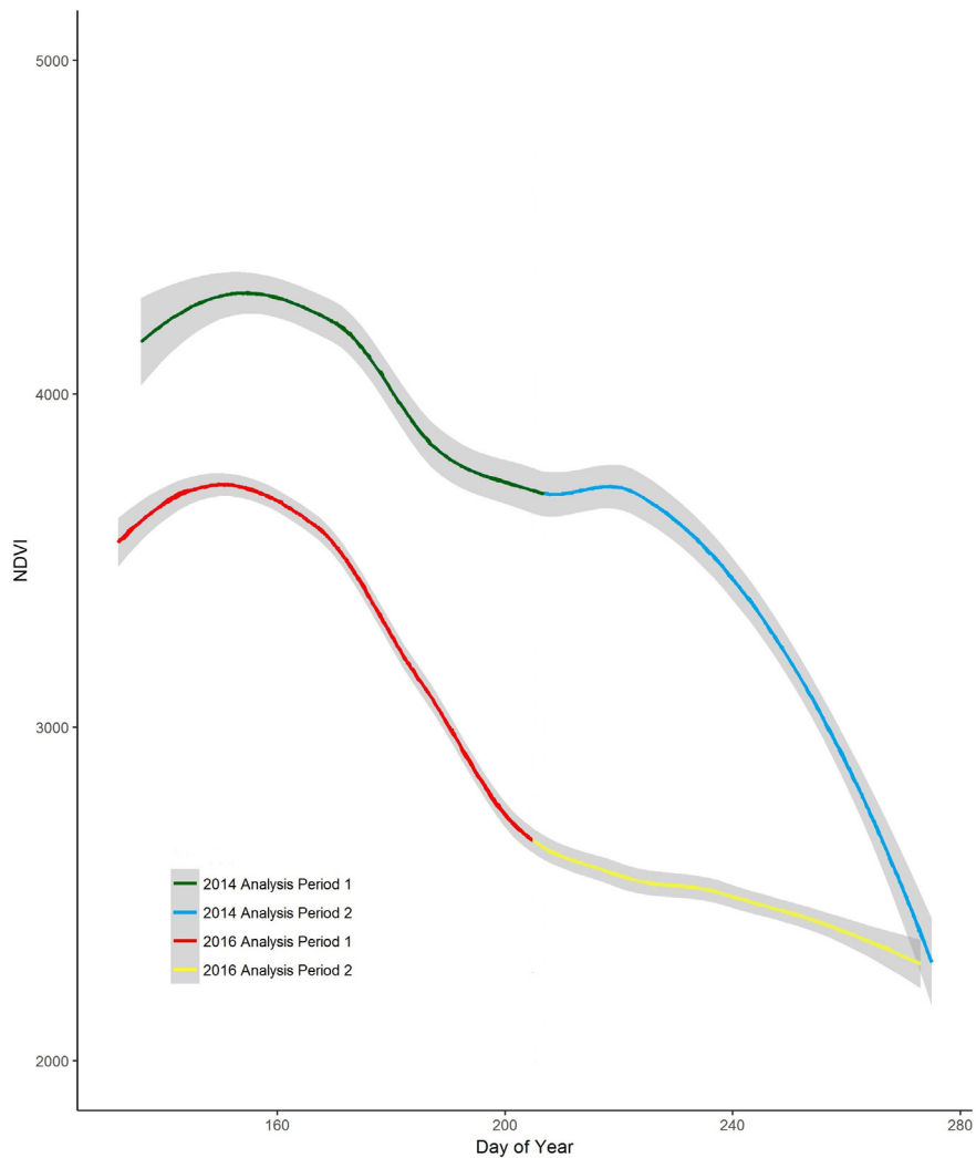
Figure 1. Temporal patterns of greenness as measured by the normalized difference vegetation index (NDVI) averages across the Central Plains Experimental Range in eastern Colorado during 2014 and 2016. Lines are smoothed trend lines fit to the data using the loess method. Cattle grazing distribution was measured during 15 May to 2 October 2 in 2014 and from 12 May to 30 September 30 in 2016.
