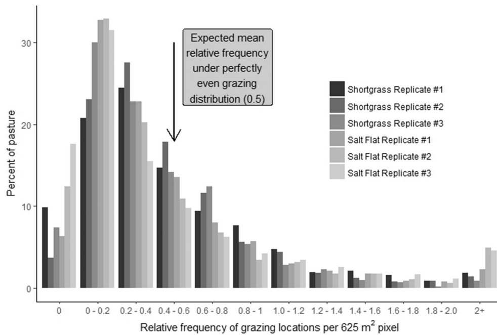
Figure 2. Histogram illustrating the percent area of each of six study pastures experiencing varying relative frequencies of cattle grazing locations in the shortgrass steppe of eastern Colorado. Grazing frequency distributions are shown for each of three pastures containing only shortgrass vegetation and each of three pastures that contained both shortgrass and saltgrass vegetation. For each pasture, the expected mean relative frequency of cattle grazing locations per pixel under perfectly even grazing distribution is 0.5.
