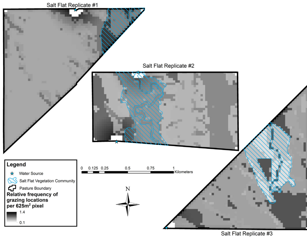
Figure 7. Predicted variation in the relative frequency of grazing locations for cattle in three pastures containing varying amounts of salt flat vegetation in eastern Colorado. See Table 3 for measures of the abundance of C 4 saltgrasses within the area mapped as a salt flat vegetation community in each replicate. Note the variation from strong selection of salt flat vegetation in replicate 1 to strong salt flat avoidance in replicate 3.
