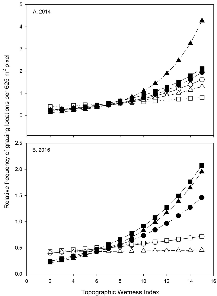
Figure 3. Relative frequency of grazing locations as a function of the topographic wetness index (TWI) per pixel ( 625 \text{ m}^2 ) for the first half of the growing season (analysis period 1; open symbols) and the second half of the growing season (black symbols) for each of three pastures encompassing shortgrass vegetation in eastern Colorado. Cattle grazing distribution response to TWI increased substantially relative to the first half of the growing season in both a wet yr (2014; A ) and a dry yr (2016; B ). Symbol shapes show the same pasture in any given year and season.
