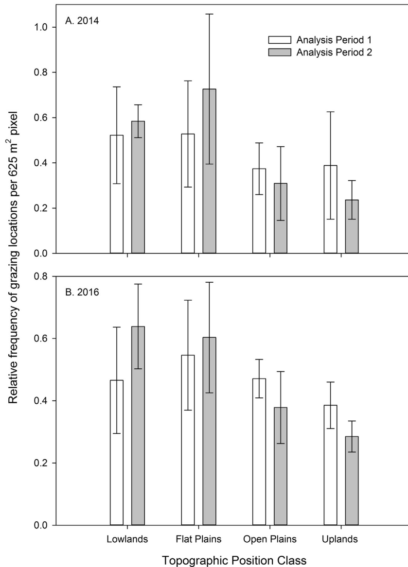
Figure 4. Variation in the mean predicted relative frequency of grazing locations per pixel (and 95% confidence intervals derived from models for 3 different pastures) for each of four topographic position classes in the shortgrass steppe of eastern Colorado during 2014 (A) and 2016 (B). White bars show predicted grazing frequency for the first half of the growing season (analysis period 1), and gray bars show the second half of the growing season (analysis period 2). See Figure 1 for temporal patterns in vegetation greenness during these analysis periods in both years.
