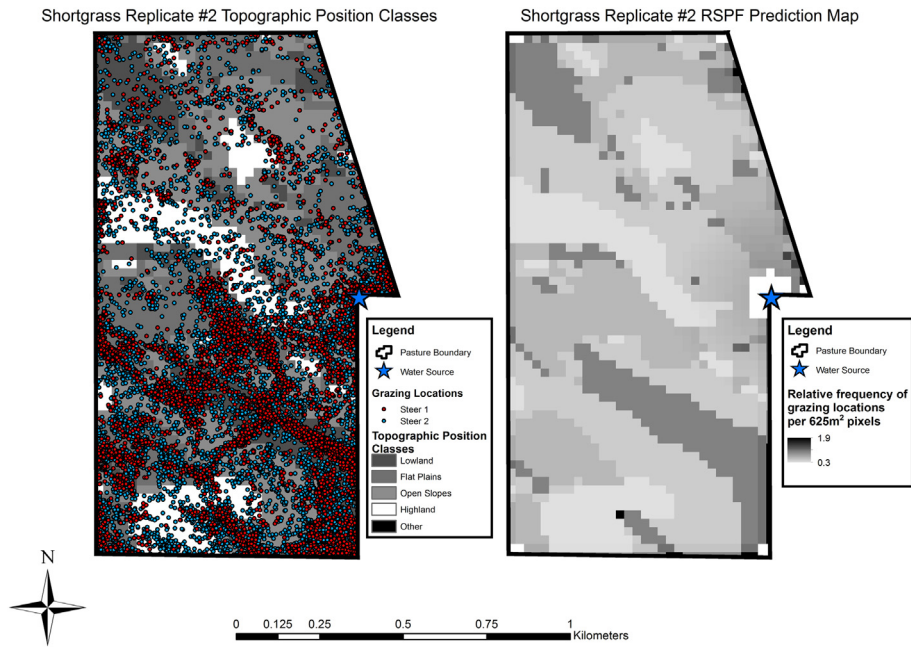
Figure 5. Example of grazing location distribution for two steers in relation to topographic position classes in a pasture encompassing shortgrass vegetation in eastern Colorado during the second half of 2016 (map on left) and the predicted resource selection probability function based on the average of models from both steers as a function of topographic classes. For both steers, the model showed strong selection for lowlands and flat plains relative to the highlands of open slopes. See Table 1 for the definition of “other” topographic position, which was rare throughout the study area.
