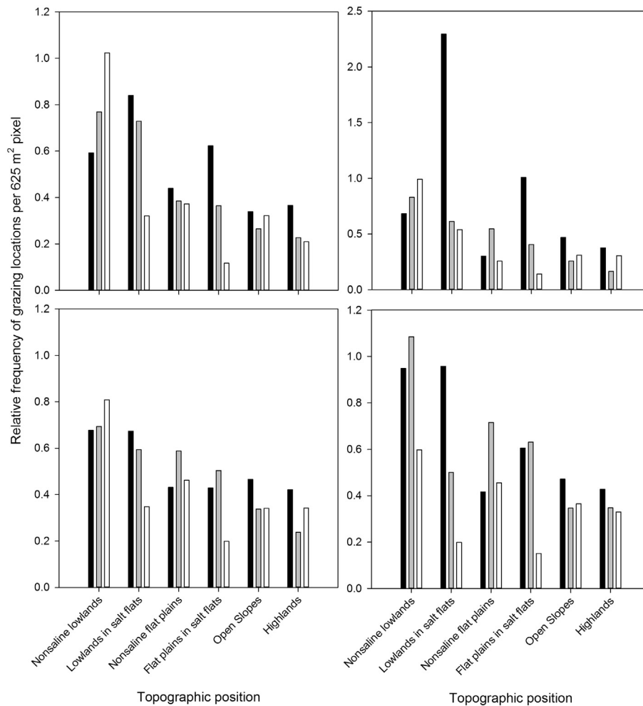
Figure 6. Predicted relative frequency of grazing locations per pixel in relation to topographic position classes and the presence/absence of salt flat vegetation in lowlands and flat plains in the shortgrass steppe of eastern Colorado during 2014 (upper panels) and 2016 (lower panels), separately for the first half of the growing season (left panels) and second half of the growing season (right panels). See Figure 1 for temporal patterns of vegetation greenness during these study periods. Each shade shows prediction values based on mean models fitted to two different steers for each of three pastures containing both shortgrass and salt flat vegetation.
