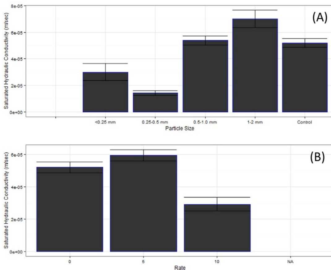
Figure 1. Comparing the impact of particle size (A) and amendment application rate (B) on soil hydraulic conductivity. Because of the similarity in the response of the biochar and raw biomass particles, the results were pooled across material type.
