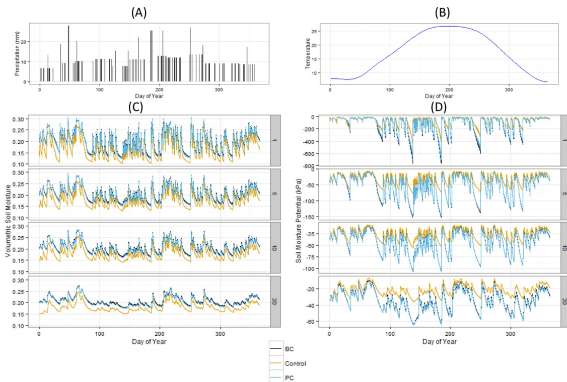
Figure 2. Predicted precipitation (A) and air temperature (B) for Florence, SC, USA, which were used as inputs to the STM2 model to simulate a 10% (w/w) addition of <0.25 mm particle-size biochar (BC) and pine chip (PC) amendments to a sandy loam soil (control) for four different depths (1, 5, 10, and 20 cm; labeled in the gray margins of the graphs) illustrating volumetric soil moisture (C) and soil moisture potential (kPa) (D).
