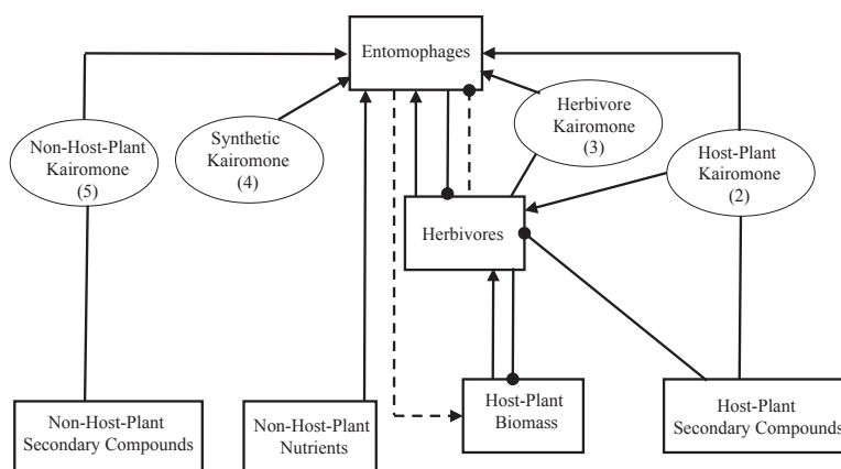
Fig. 2. Diagram of kairomone sources (designated by ovals) in field crop host plant-herbivore-entomophague interactions (designated by rectangles): Solid lines indicate direct effects and dashed lines, indirect effects. Arrows indicate positive effects and circle heads, negative effects. Numbers in parentheses designate sections of report where the kairomone types are discussed.
