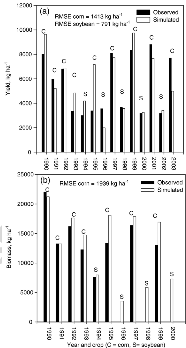
Fig. 1. Observed and simulated (a) grain yield, and (b) biomass of corn and soybean crops from 1990 to 2003. Observed data for 1993, 1994 and 1995 were not considered for calibration, but the model was run continuously from Jan 1, 1978 to 31 Dec., 2003. C = corn, S = Soybean. There was only one observation for soybean biomass, hence RMSE was not calculated. (RMSEs shown in the figures do not include data for 1993, 1994 and 1995).
