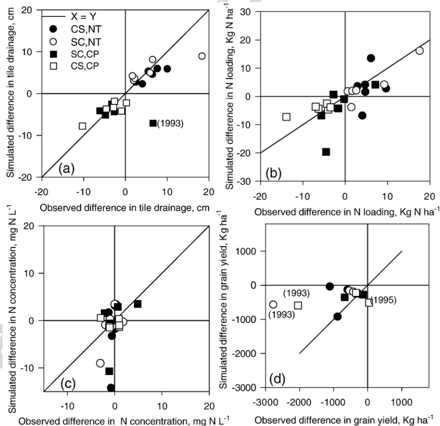
Fig. 6. Simulated and measured management effects between SA and LSNT (SA–LSNT) for CS and SC under CP and NT on tile drainage, N loading in tile drainage, flow weighted N concentration in tile drainage, and grain yield. (SA = single N application at pre-plant, LSNT = split dose N application at pre-plant and in late-spring based on late-spring soil N test, CP = chisel plow, NT = no till, CS = corn–soybean rotation with corn during even years, and SC = soybean–corn rotation with corn during odd years).
