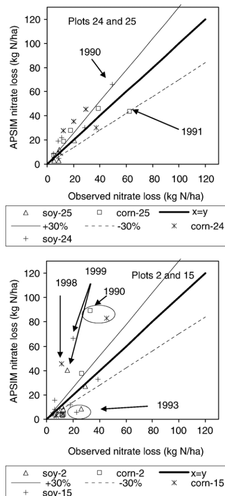
Fig. 6. Observed and APSIM simulated yearly nitrate-N loss in tile drains.
