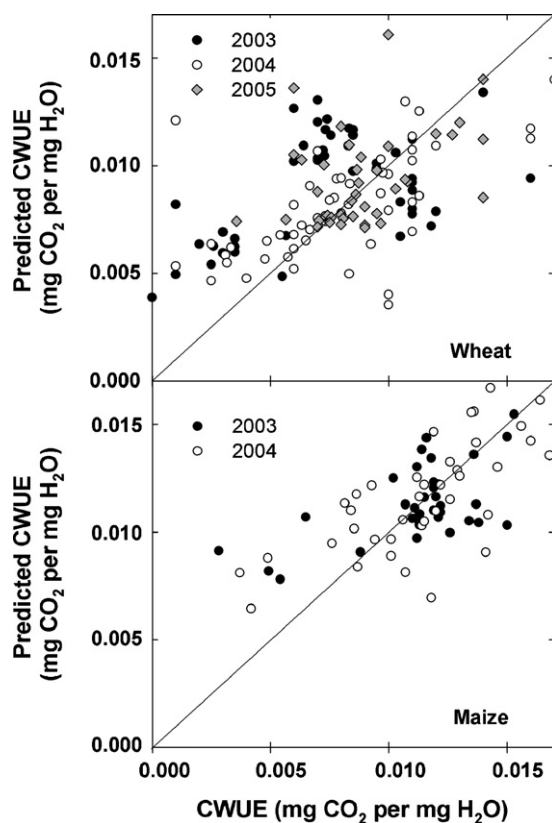
Fig. 8. Comparison of observed canopy water use efficiency (CWUE) over wheat and maize with values of CWUE predicted by multiple linear regressions using values of crop water stress index and net radiation.
