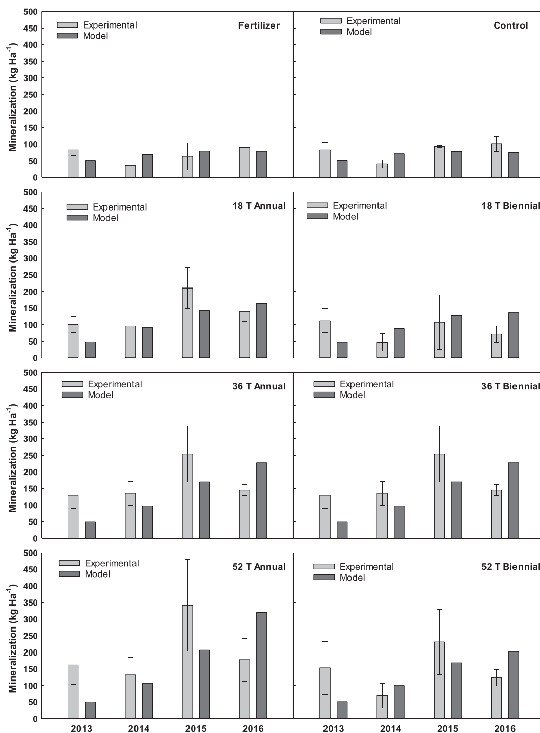
Fig. 4. Experimental and model results for \text{NO}_3\text{-N} mineralized. The experimental N mineralized represents the top 30 cm of the soil profile. The crop rotation is wheat, potato, barley, and sugar beet for 2013, 2014, 2015, and 2016, respectively. The error bars represent one standard deviation.
