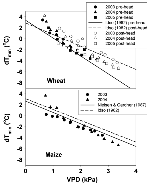
Fig. 1. Relationship between vapor pressure deficit (VPD) and minimum canopy-air temperature difference ( dT_{min} ) as calculated by Eq. (2) (Jackson energy balance method) over wheat and maize canopies. The data points are from half-hourly average values taken between 1230 and 1500 when net radiation was greater than 500 W m -2 .
