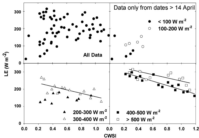
Fig. 5. Relationship between Crop Water Stress Index (CWSI) and latent heat flux (LE) for winter wheat on the North China Plain, 2003. Data are from half-hourly values from 1230 to 1500 local time that were then averaged by 0.1 CWSI classes and separated by net radiation class.
