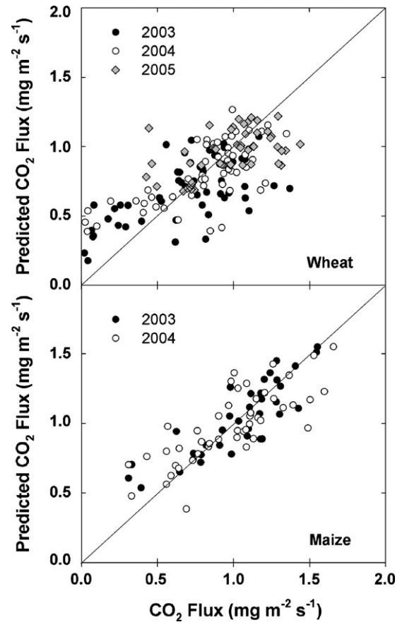
Fig. 7. Comparison of observed CO 2 flux (Fc) over wheat and maize with values of Fc predicted by multiple linear regressions given in Table 3 using values of crop water stress index and net radiation.
