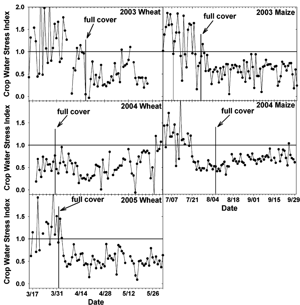
Fig. 3. Crop Water Stress Index for wheat (2003–2005) and maize (2003–2004).
