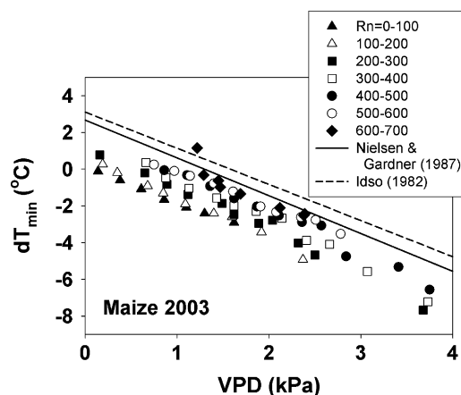
Fig. 2. Relationship between vapor pressure deficit (VPD) and minimum canopy-air temperature difference ( dT_{min} ) as calculated by Eq. (2) (Jackson energy balance method) over a maize canopy in 2003. The data points are from half-hourly average values taken between 1230 and 1500 and are separated by net radiation class.
