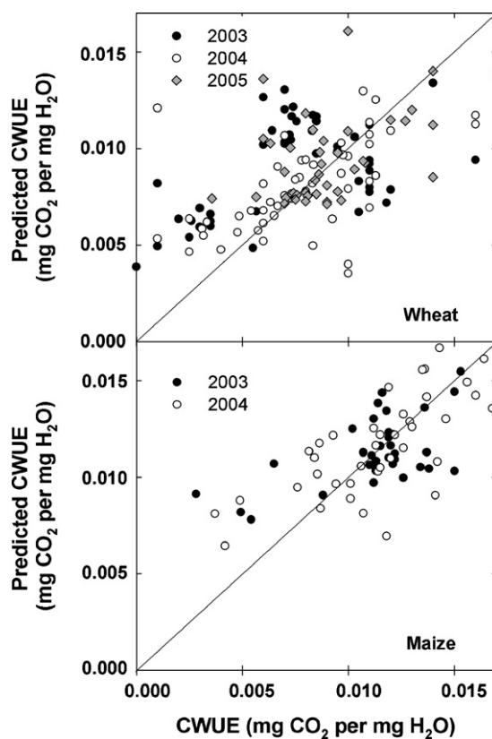
Fig. 8. Comparison of observed canopy water use efficiency (CWUE) over wheat and maize with values of CWUE predicted by multiple linear regressions given in Table 3 using values of crop water stress index and net radiation.
