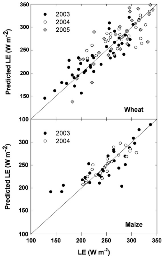
Fig. 6. Comparison of observed latent heat flux (LE) over wheat and maize with values of LE predicted by multiple linear regressions given in Table 3 using values of crop water stress index and net radiation.
