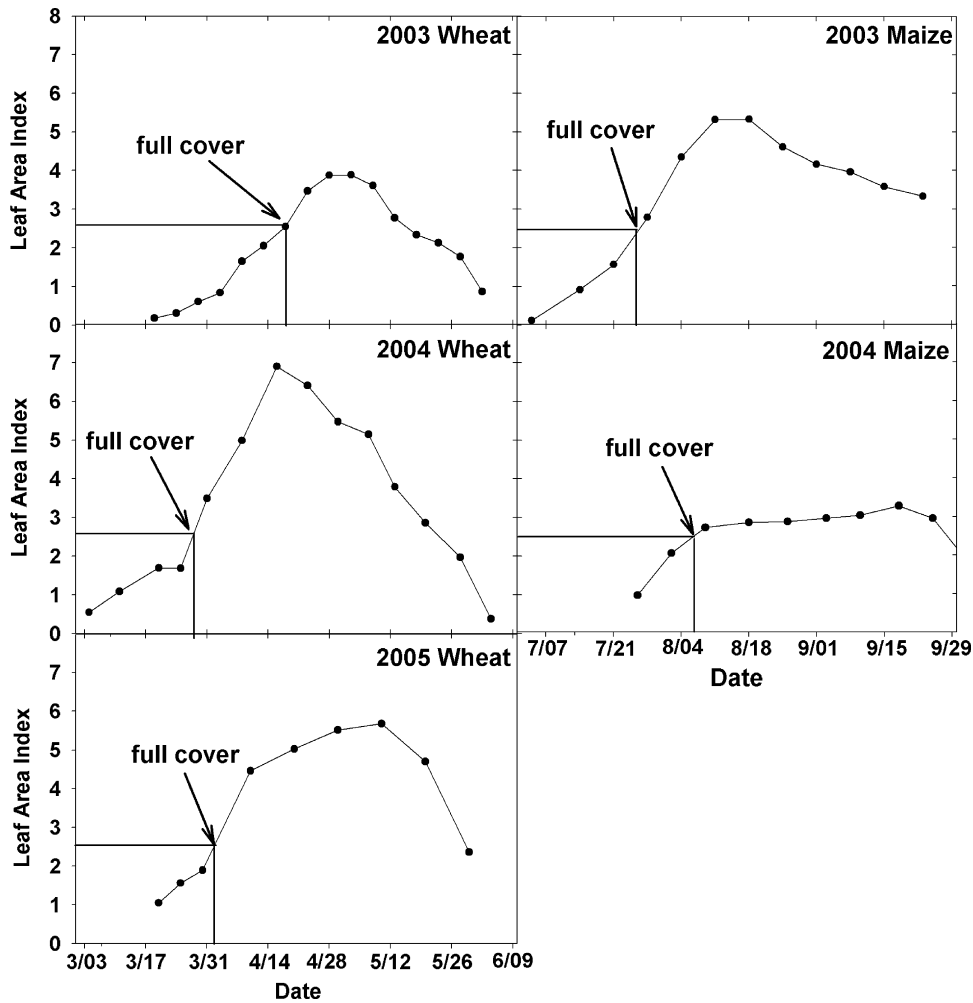
Fig. 4. Winter wheat and maize leaf area index development from 2003 to 2005.
