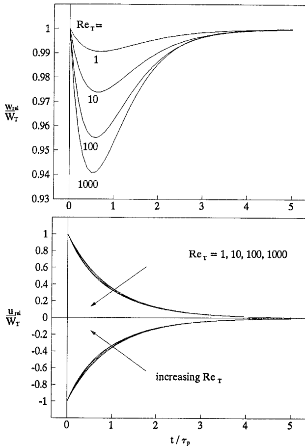
FIG. 5. Response of a particle to a step change of horizontal relative motion.
