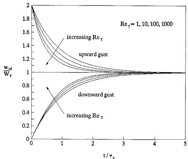
FIG. 6. Response of a particle to a step change of vertical relative motion.
