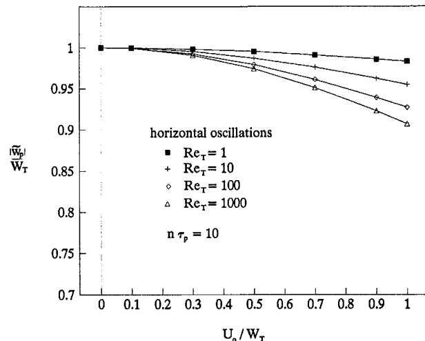
FIG. 9. Cycle-averaged settling velocity within a horizontally oscillating fluid as a function of scaled oscillation amplitude and Re_T .
