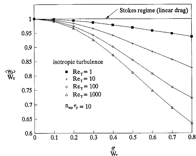
FIG. 13. Ensemble-averaged settling velocity within simulated isotropic turbulence as a function of \sigma/W_T and Re_T .
