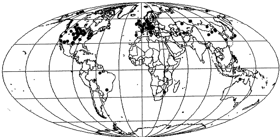
Figure 1. Geographical distribution of the 118 nonforest flux-tower sites considered in this study.
