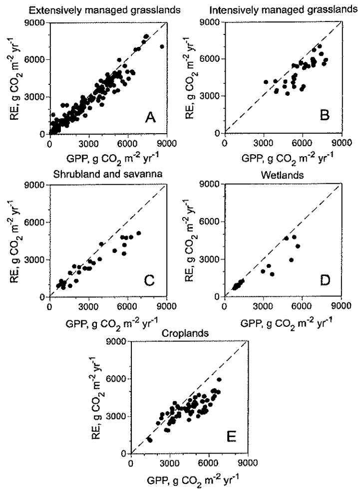
Figure 10. Scatter plots of the ecosystem respiration (RE) vs. gross primary production (GPP) values for various types of nonforest ecosystems: A , extensively managed grasslands; B , intensively managed grasslands; C , shrublands and savanna; D , wetlands; E , croplands.
