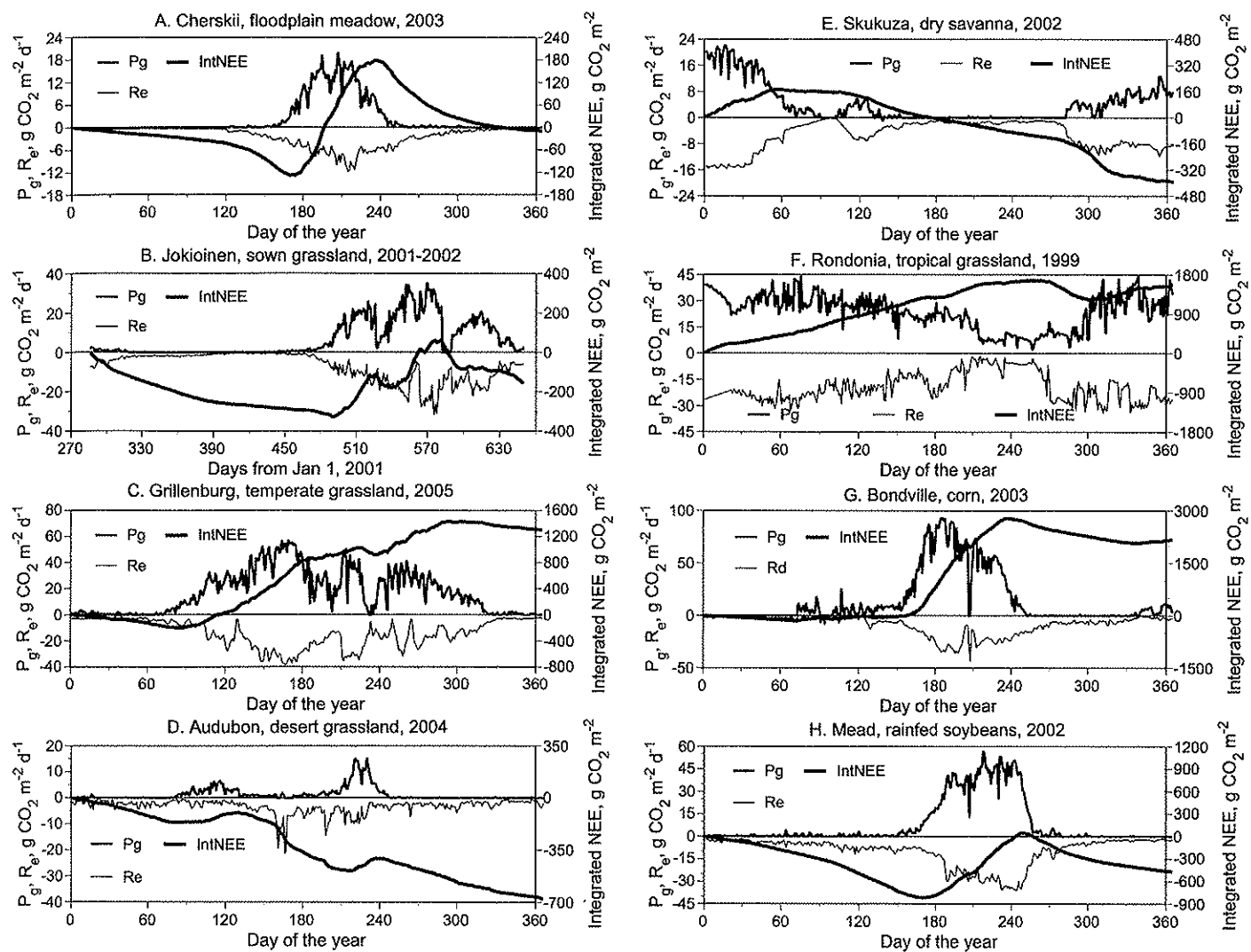
Figure 7. Seasonal dynamics and annual budgets of gross primary productivity, P_g(t) , total ecosystem respiration, R_e(t) , and integrated net ecosystem \text{CO}_2 exchange, \text{IntNEE}(t) , for selected nonforest sites and years: A , floodplain meadow, Cherskii, 2003; B , sown northern temperate grassland, Jokioinen, 2001–2002; C , temperate grassland, Grillenburg, 2005; D , desert grassland, Audubon Ranch, 2004; E , dry savanna, Skukuza, 2002; F , tropical grassland, Rondonia, 1999; G , maize crop, Bondville, 2003; H , soybean crop, Mead, 2002.
