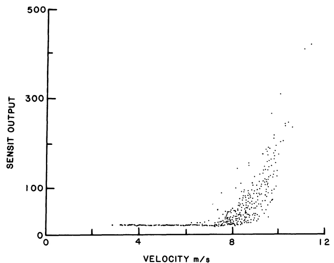
Figure 4—SENSIT output for a smooth, bare, fine, sandy-loam soil surface for various wind velocities on the 11 March 1988 storm.
