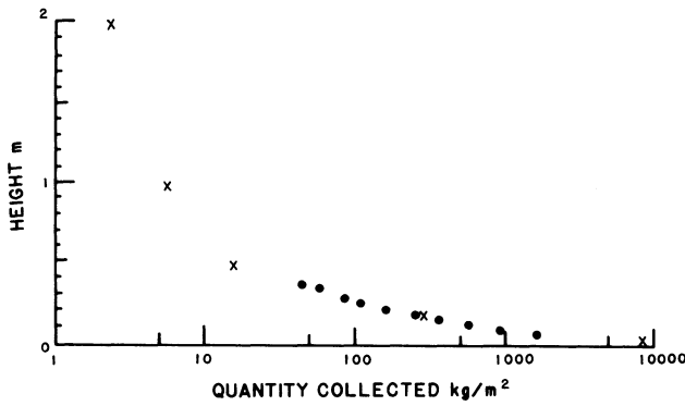
Figure 2—Vertical mass for cluster “J”, 11 March 1988. Quantity collected is on log scale. Data From Modified BSNE “Vories” samplers are circles, the x are from cluster “J”.
