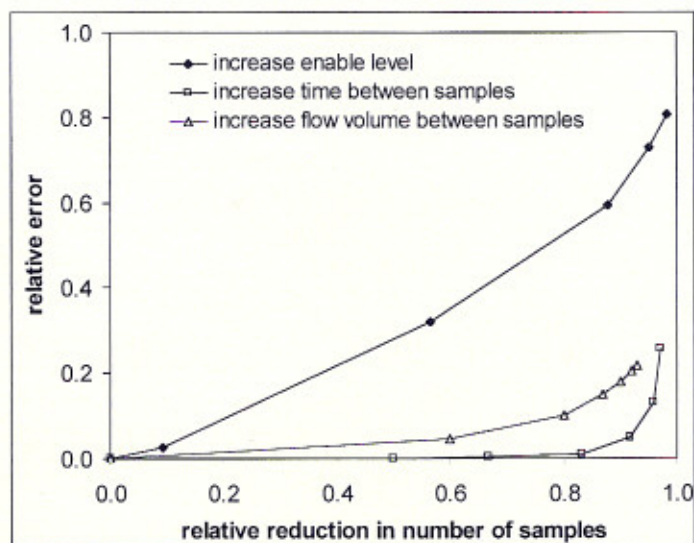
Figure 4. Comparison of relative errors for various sampling strategies to manage the number of samples.
