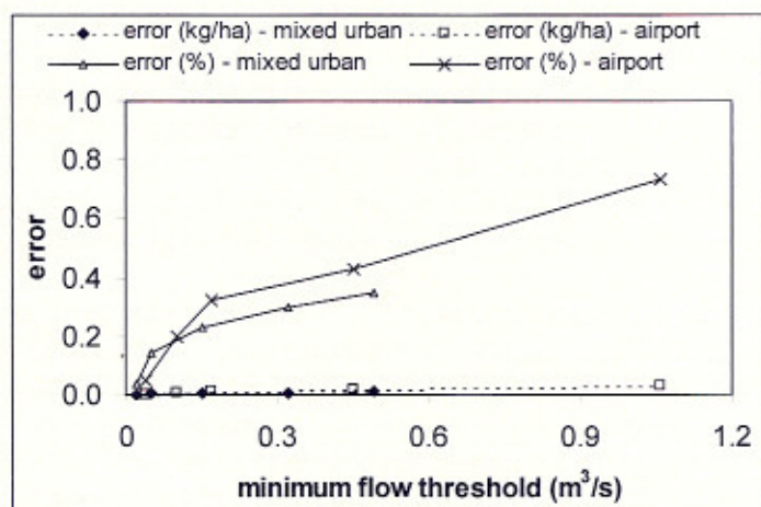
Figure 3. Relative and absolute errors the larger urban watersheds for various minimum flow thresholds.
