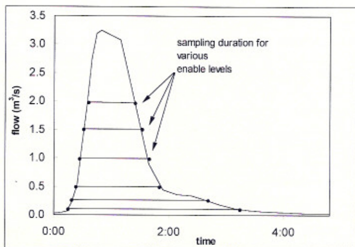
Figure 1. Sample storm illustrating duration of sample collection for various enable levels.
