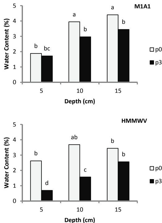
Figure 12. Vehicle \times pass \times depth interactive effects for soil water content in the M1A1 and HMMWV tracks at Fort Benning. Bars with different letters are significantly different ( p \leq 0.05 ).
