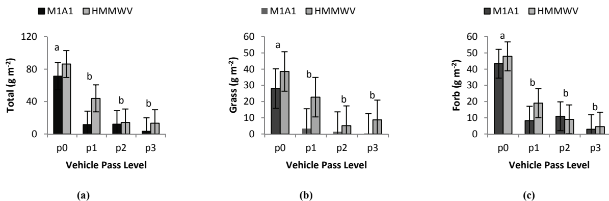
Figure 3. Influence of vehicle pass intensity level on (a) total, (b) grass, and (c) forb biomass across all sampling locations: p0 is from an untrafficked location, and p1, p2, and p3 represent 1, 5, and 10 passes with the M1A1 and 10, 25, and 50 passes with the HMMWV, respectively. Bars with different letters are significantly different ( p \leq 0.05 ) for the main effect of vehicle pass.
