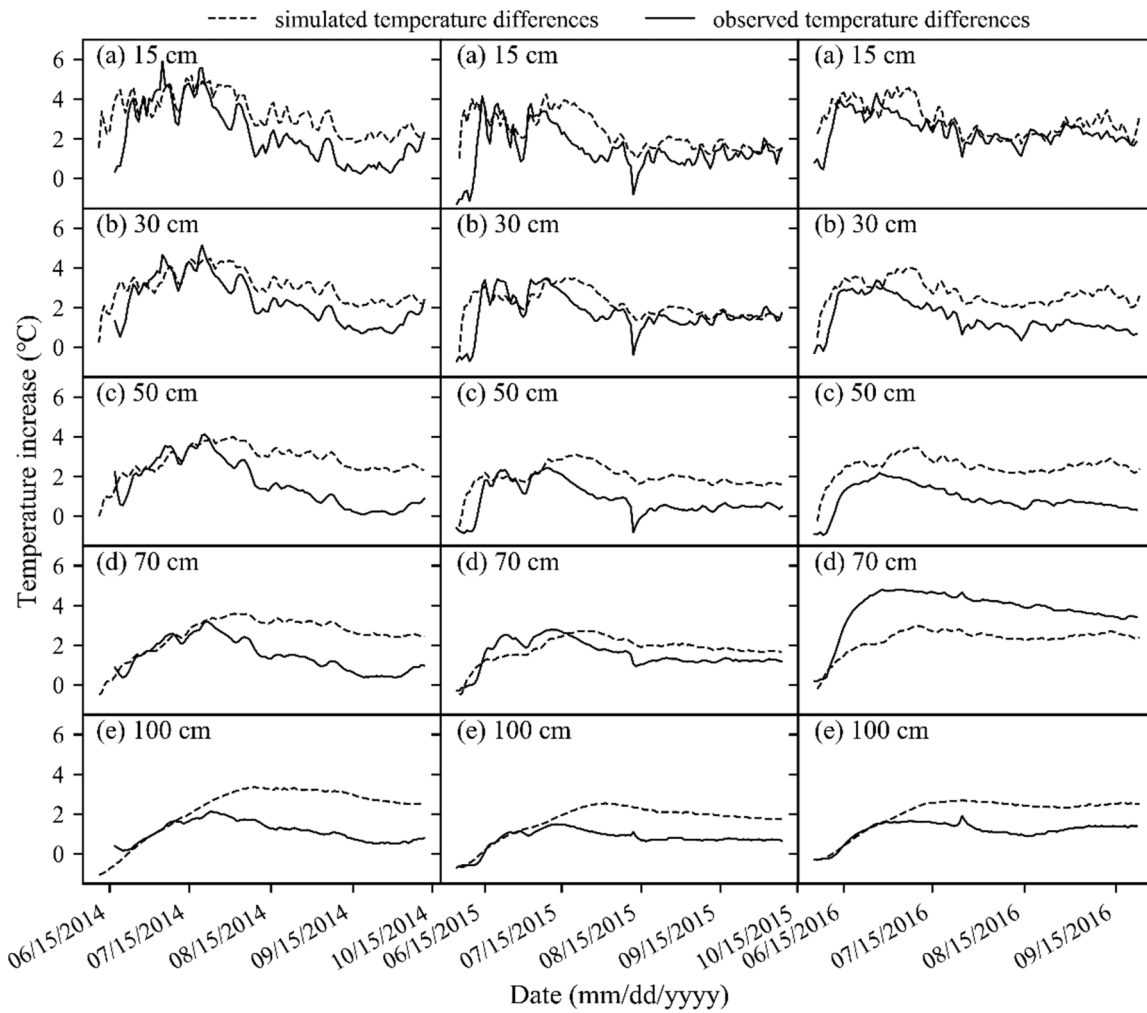
Fig. 8. Simulated temperature differences (°C) and observed temperature differences (°C) between TPM and CK treatments at 15, 30, 50, 70, 100 cm soil depths at Yangling, China. At each soil depth, temperature differences were calculated by simulated or observed soil temperature with plastic mulch minus that without plastic mulch.
