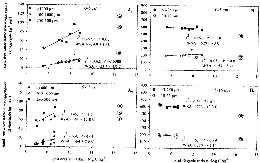
Fig. 4. Relationship between sand-free water-stable aggregates (WSA) and whole-soil organic C ( \text{Mg C ha}^{-1} ) as affected by different cropping intensities and tillage within the 0- to 5-cm depth for (A 1 ) macroaggregates and (B 1 ) microaggregates, and the 5- to 15-cm depth for (A 2 ) macroaggregates and (B 2 ) microaggregates. The regression lines for A 1 and A 2 group large macroaggregates (>1000 and 500–1000 \mu\text{m} ) fractions together for analysis, where different symbols identify each aggregate size class. The symbols that are circled represent the relationship between sand-free WSA and SOC from soils collected at the reference prairie site and are included for reference purposes only. The prairie data were not included in the regression analysis.
